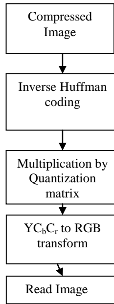
Figure 4-Hybrid model Reconstruction Flow
