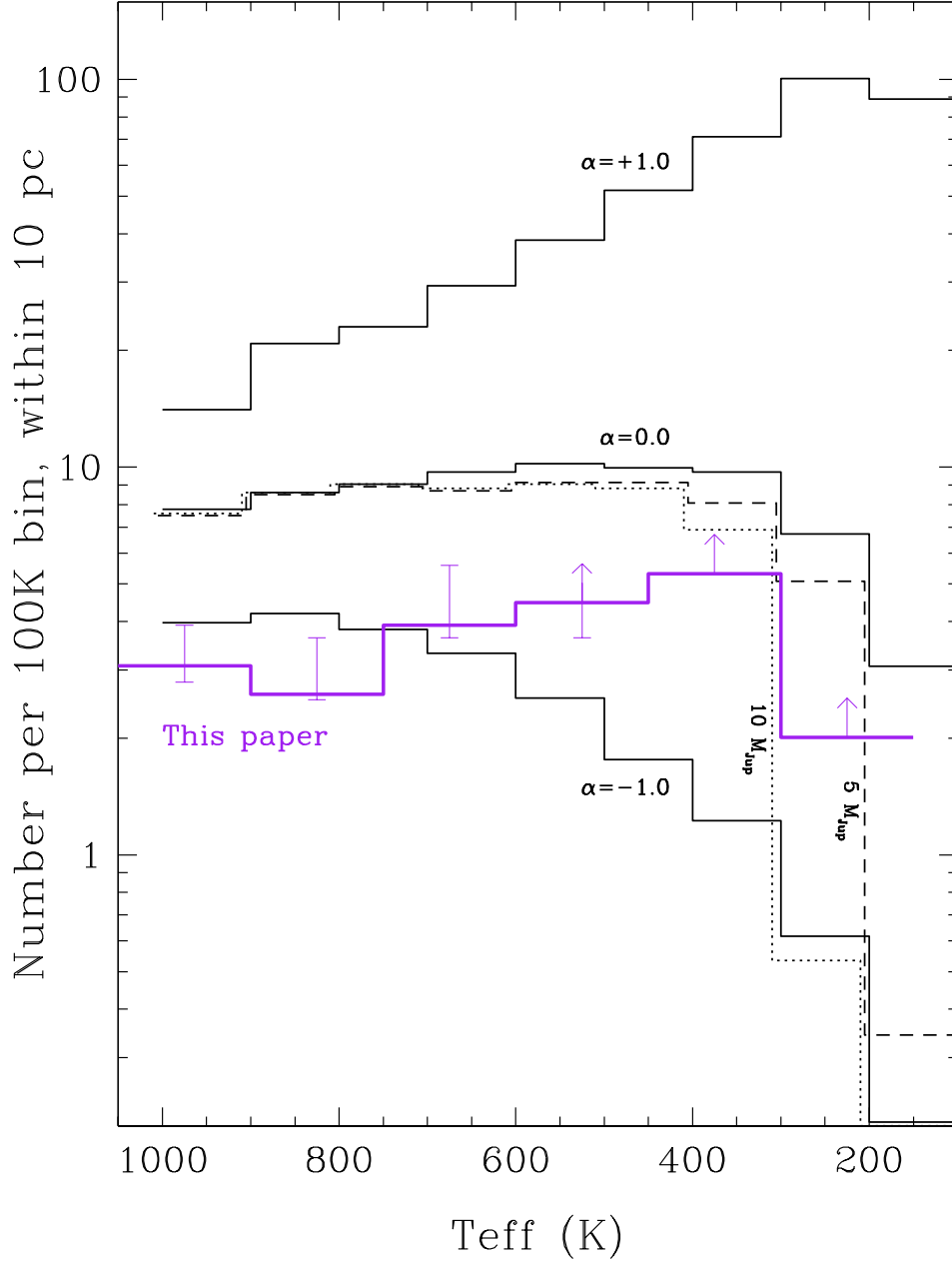
Fig. 14.— The predicted number of brown dwarfs within 10 pc for three different power-law mass functions ( dN/dM \propto M^{-\alpha} ) with \alpha = -1, 0 , and +1 (solid black) having a minimum formation mass of 1 M_{Jup} . Also shown for the \alpha = 0 model is the predicted number of brown dwarfs if a minimum formation mass of 5 M_{Jup} (dashed black) or 10 M_{Jup} (dotted black) is assumed. These simulations are from Burgasser et al. (2004, 2007). Space densities using our full accounting of objects in the immediate Solar Neighborhood (Tables 8 and 9) are shown by the heavy purple line.
