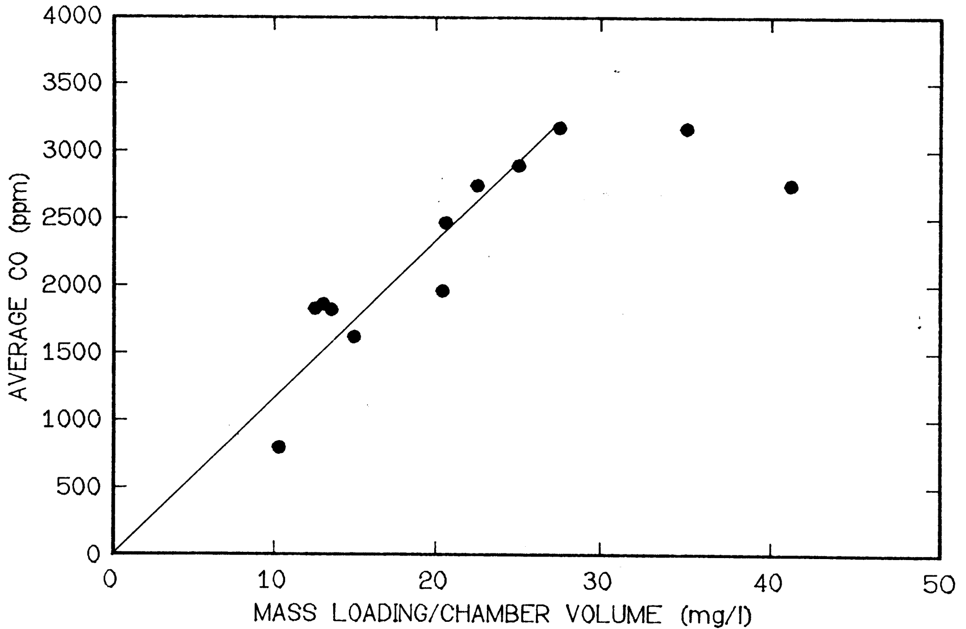
Figure 15. Overloading of furnace capacity as seen with non-flaming decomposition of Douglas fir in the NBS large furnace. Small furnace had similar results.
