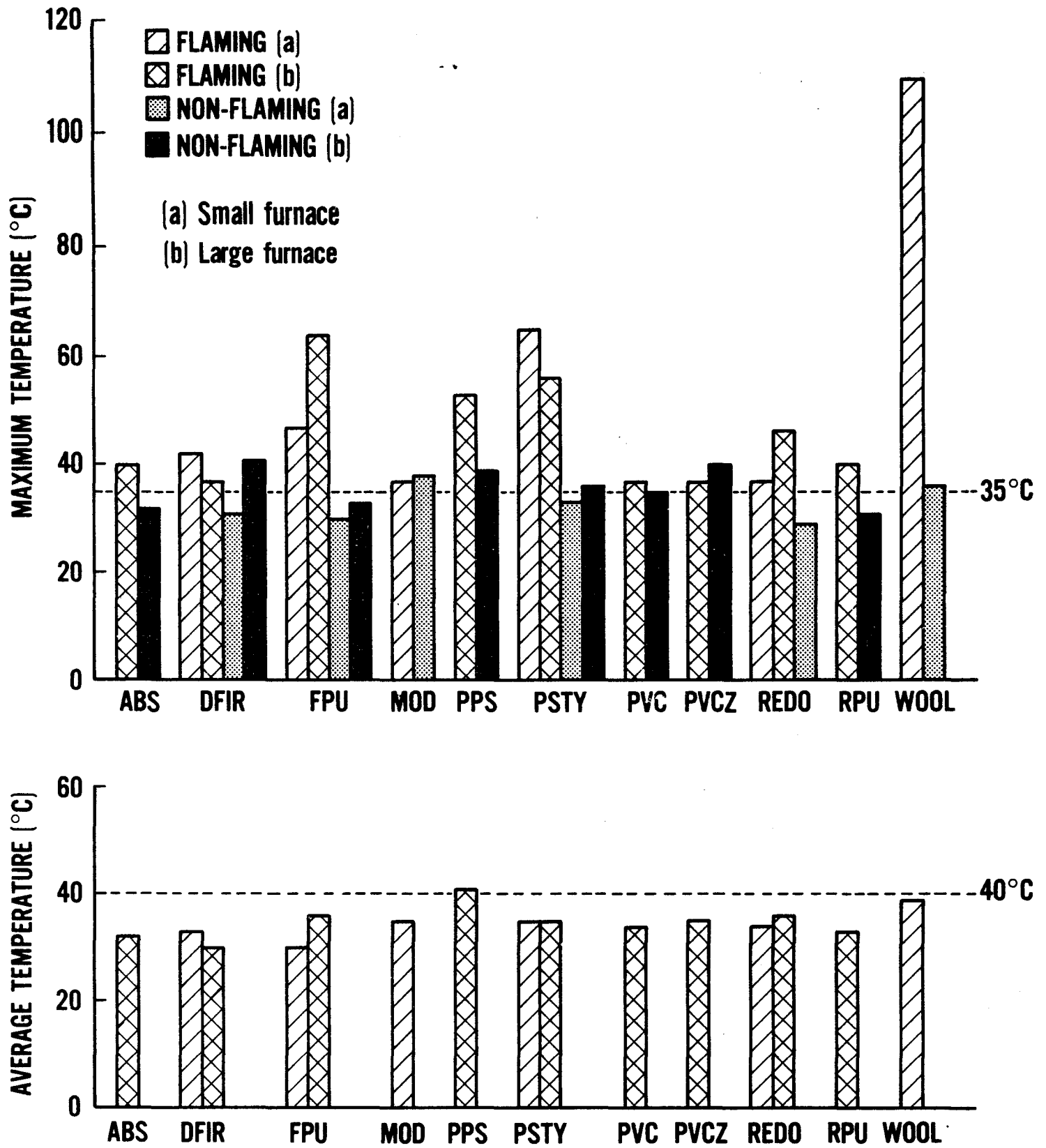
Figure 8. NBS exposure chamber temperatures at animal nose levels. Top: Maximum temperatures. Bottom: Average temperatures.
