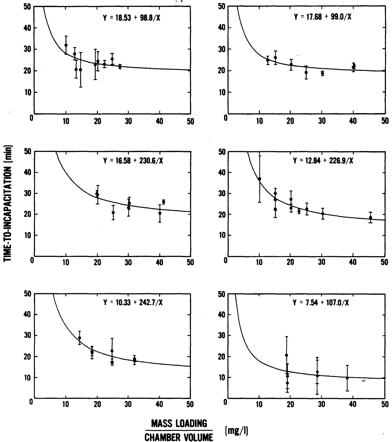
Figure 20. Time-to-incapacitation vs mass loading/chamber volume hyperbolas for Douglas fir in the non-flaming mode from six laboratories. (Symbols refer to the mean and standard deviation of the times-to-incapacitation of the 6 animals tested at each mass loading.)
