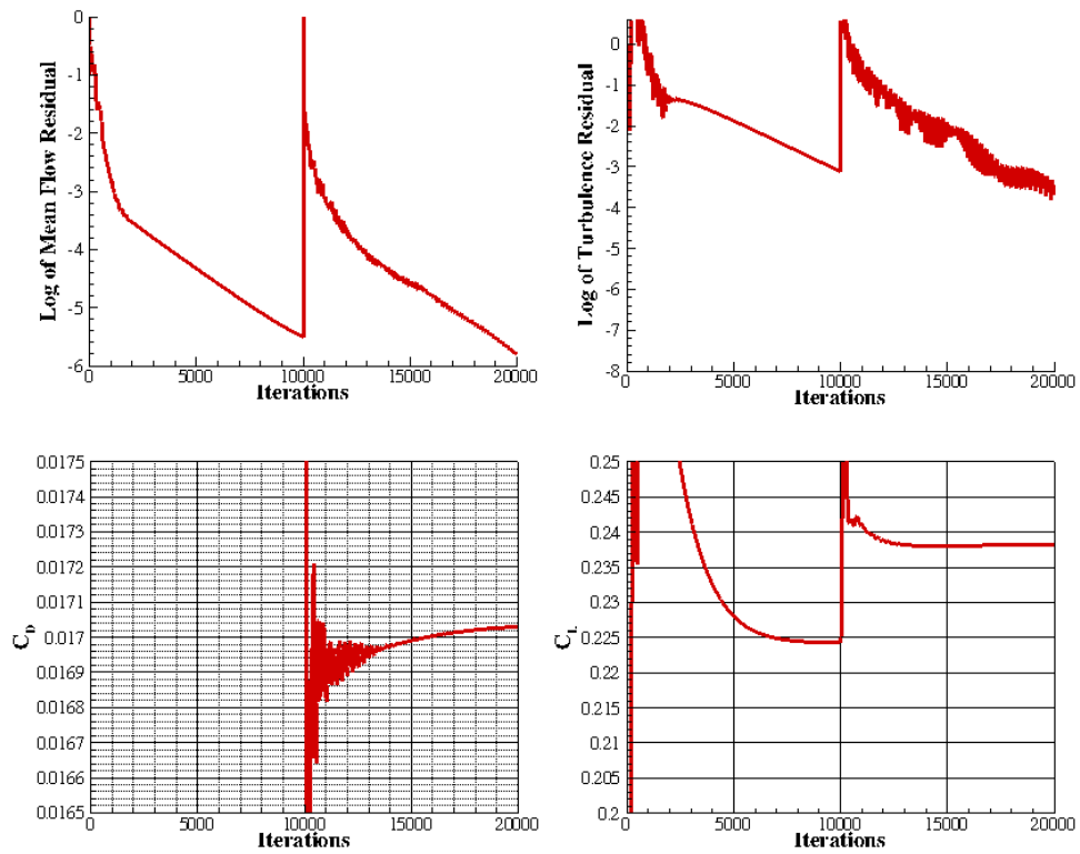
Figure 17. WBT0ss convergence history, M_{co}=0.85 , \alpha=1.0^\circ , Re_c=5 million. (Note: spatial accuracy of computations 1 st order for first 10000 iterations then set to 2 nd order)
