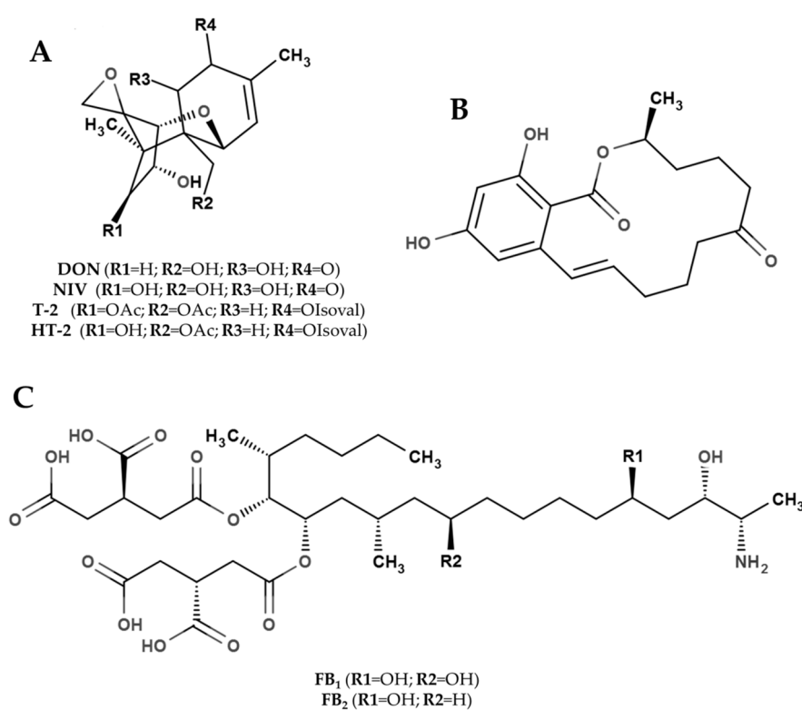
Figure 1. Chemical structure of the main Fusarium mycotoxins. (A) Trichothecenes; (B) Zearalenone; (C) Fumonisins; OAc = acetyl function; OIsoval = isovalerate function.
