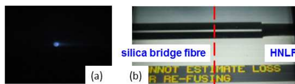
Fig.2 (a) Near-field image of 1.55 \mu\text{m} laser guiding from output end of lead silicate glass HNLf butt-coupled with silica bridge fibre on splicer. (b) Photograph of spliced lead silicate glass HNLf sample with silica bridge fibre.
