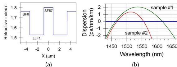
Fig.1 (a) W-type index profile of lead silicate glass HNLF; (b) measured dispersion profiles of two samples of lead silicate glass HNLFs
