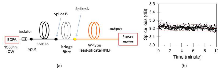
Fig.3 (a) Schematic of power test on spliced fibre sample. Note that length of HNLf is no more than 1meter to minimize nonlinear effect. (b) Stability of splice loss of splice A (between HNLf sample 1 and bridge fibre UHNA3) when 1.8W power is directly attenuated on splicer A.
