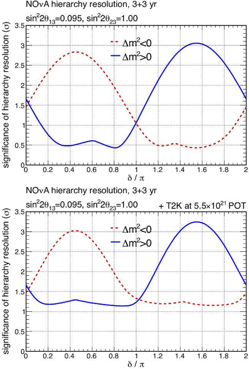
Figure 1: Expected significance for resolution of the neutrino mass hierarchy, shown as a function of the CP phase \delta_{CP} , for NOvA after 6 years of running (top plot), and the improvement when combined with the anticipated final T2K data sample (bottom plot). The two curves correspond to the two possible hierarchies. Figure kindly provided by the NOvA Collaboration.
