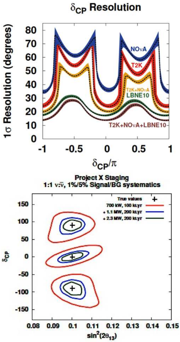
Figure 2: Anticipated precision for the determination of the CP phase \delta_{CP} and the mixing parameter \sin^2 2\theta_{13} . Top plot shows, as a function of \delta_{CP} , how the resolution on \delta_{CP} is expected to improve with time as future experiments run and deliver results. Bottom plot shows how the precision in determining the point in (\delta_{CP}, \sin^2 2\theta_{13}) -space improves with statistics. See C. Adams et al. [6]. Figure kindly provided by the LBNE Collaboration.
