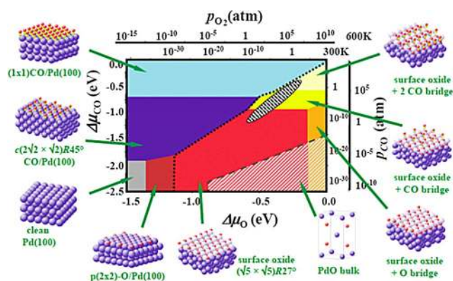
Figure 9. Surface phase diagram for a Pd(100) model catalyst in “constrained” thermodynamic equilibrium with an environment consisting of O 2 and CO. Phases involving the pristine metal termination are above the dotted line, phases involving the surface oxide are below the dotted line, while bulk-like PdO is stable at operation conditions below the dashed line. The dependence on the chemical potentials of O 2 and CO in the gas phase is translated into pressure scales at 300 and 600 K. The black hatched ellipse marks gas-phase conditions representative of technological CO oxidation catalysis, i.e., partial pressures of 1 atm and temperatures between 300 and 600 K. Adapted from Ref. [102]; available under the terms of the Creative Commons Attribution 3.0 License, Copyright 2007.
