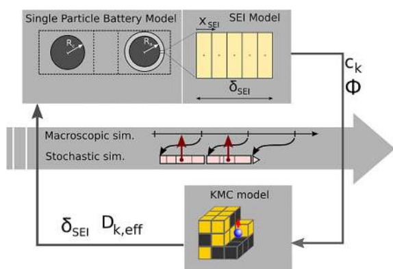
Figure 10. Multiscale model for a degrading Li ion battery: The macroscopic model contains a full battery cell model with mass and charge balances in electrolyte, electrode and degradation layer, whereas the KMC model contains the degradation kinetics with detailed sorption, reaction, surface diffusion processes and Li intercalation. The exchange of states and constants in each time step between the deterministic and stochastic model requires step size synchronization and filtering of KMC output. [113]
