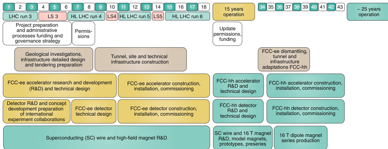
Fig. 1 | Technical schedule of the FCC integrated project. The FCC project extends over 70 years with a starting date (year 1), for example, in year 2021 (ref. 18). The top two rows show the LHC and high-luminosity LHC schedule, including years of operation (numbered along the top), four data-taking periods (runs), and intermittent maintenance periods, so-called long-shutdowns (LS). In the rows below, the FCC administrative processes (in white), infrastructure activities (in grey), the FCC-ee schedule (in yellow), and the FCC-hh schedule (in green) are depicted.
