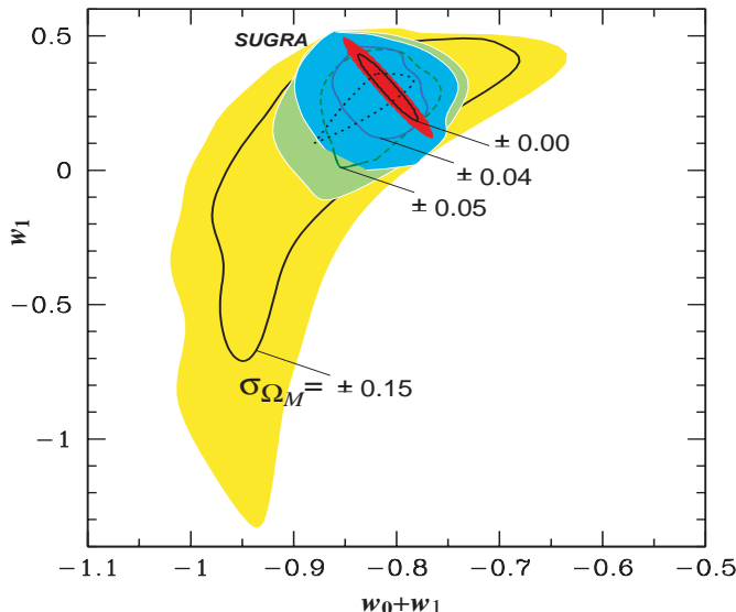
FIG. 17. Error contours of the SUGRA model with different priors on \Omega_m in the \tilde{w}_0 - w_1 plane. The solid line contours are the 39.3% joint probability regions, which project to 1\sigma errors on the axis and shaded regions represent the 68% or 1\sigma joint probabilities. The range of increasingly larger contours represents the result using prior knowledge on \Omega_m with increasingly poorer uncertainty, \sigma_{\Omega_m} = \delta\Omega_m . The unlabelled, black dotted curve corresponds to the projected- 1\sigma error contour obtained for more optimistic dataset specifications and with a prior of 0.25 \leq \Omega_m \leq 0.35 .
