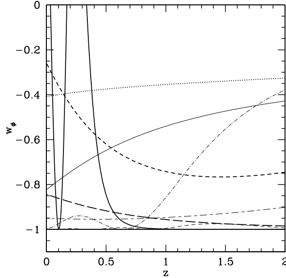
FIG. 5. The redshift evolution of equation of state factor w_\phi = p_\phi/\rho_\phi for the discussed models. The thin short dash line is the trapped minimum model, the thin dot - short dash line is from the brane inspired potential, the thin short dash - long dash line from the potential which involves two exponentials, the thick short dashed line from the periodic potential, the thick long dashed line from the pure exponential, the thick solid line from the Pseudo Nambu-Gotu Boson potential, the thin solid line from the Supergravity inspired potential, the thin long dashed line from the exponential tracker solution (underneath w = -1 ), and the thick dotted line from the inverse tracker.
