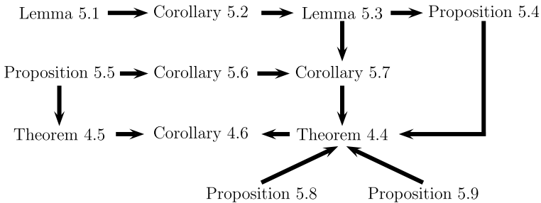
FIGURE 2. Dependencies to obtain Corollary 4.6.
