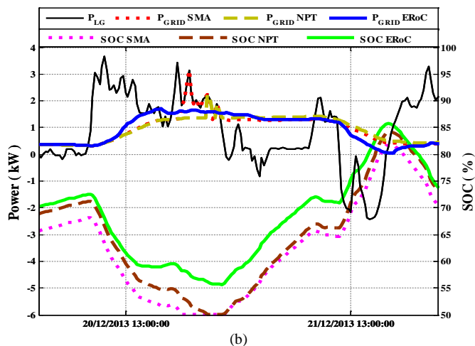
Fig. 15. Improved behavior of the proposed EMS design respect to the SMA strategy and the fuzzy EMS strategy based on MG NPT (a) improved battery SOC evolution, and (b) influence of the derivative input in the grid power profile and the battery SOC.
