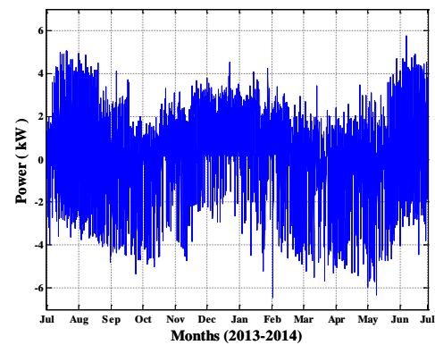
Fig. 3. Microgrid net power profile.
