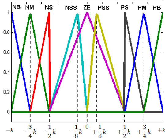
Fig. 11. Membership functions for the controller output P_{FLC}(n) .
