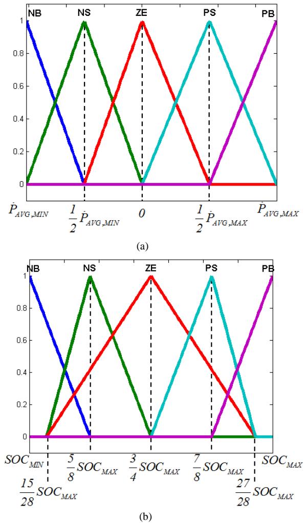
Fig. 10. Input variables membership functions (a) \dot{P}_{AVG}(n) , and (b) SOC(n) .
