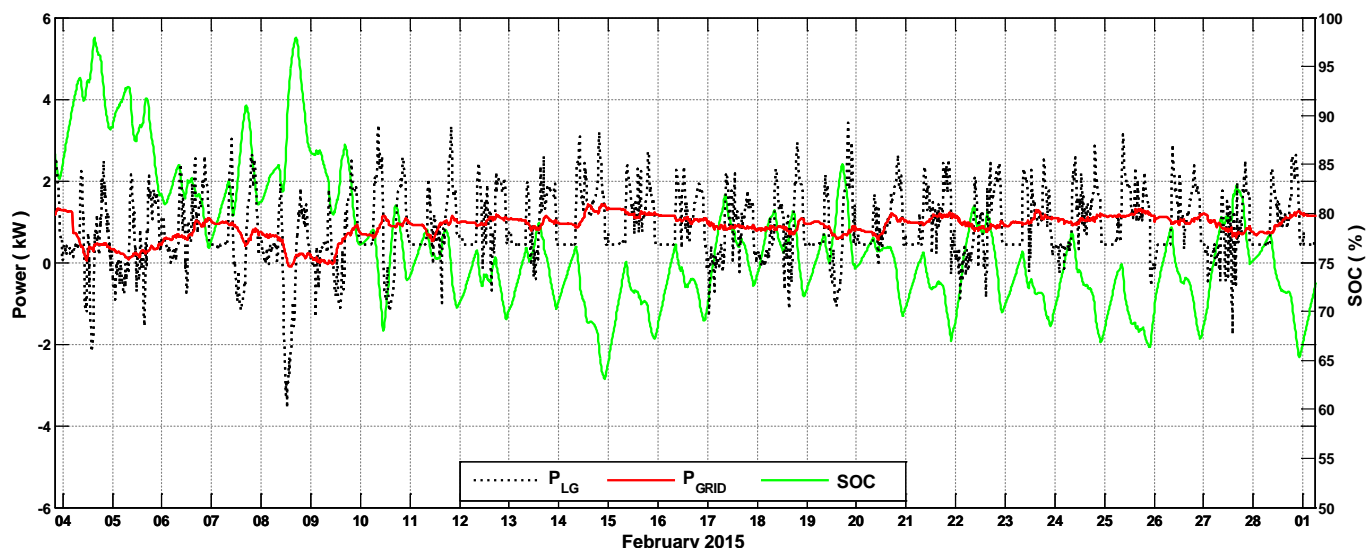
Fig. 17. Experimental results of the proposed fuzzy EMS based on MG energy rate-of-change, MG net power profile, grid power profile and battery SOC evolution.
