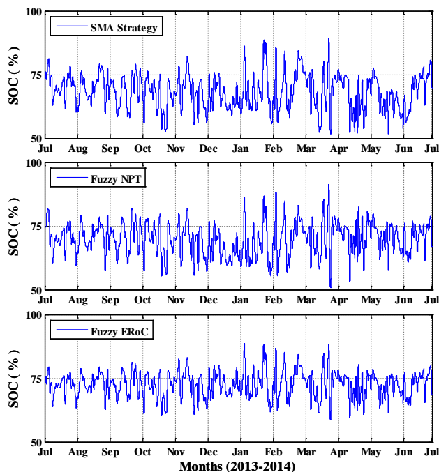
Fig. 14. Daily average profile of the battery SOC during the year under study for the SMA strategy (top), the fuzzy EMS based on MG NPT (middle), and the proposed fuzzy EMS based on MG ERoC (bottom).
