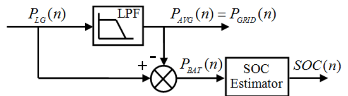
Fig. 4. Simple moving average EMS block diagram.
