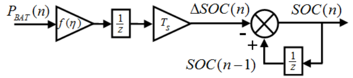
Fig. 2. Battery energy estimator block diagram.
