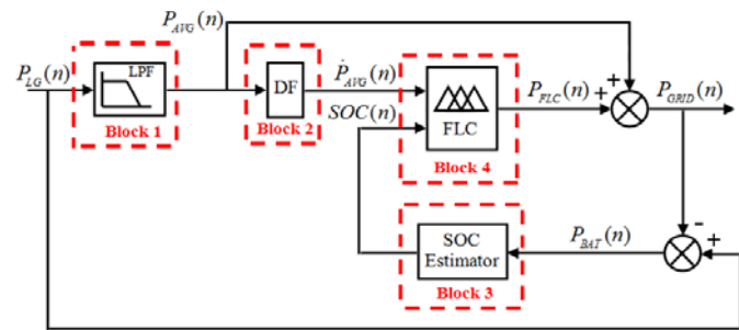
Fig. 9. Fuzzy EMS design based on MG energy rate-of-change block diagram.
