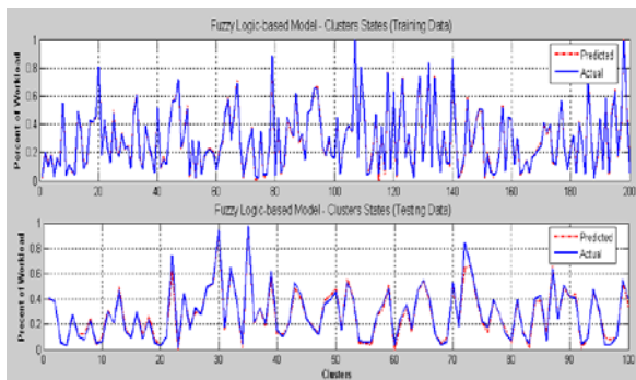
Figure 5. The fuzzy model – Cluster state (training and testing accuracy measures)
