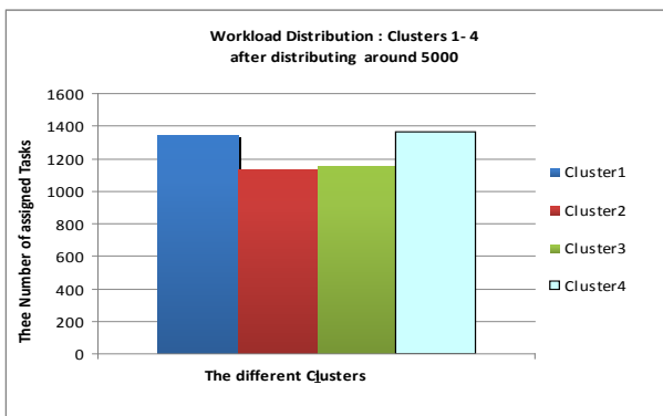
Figure 8. The workload states of the clusters after distributing the tasks by applying the proposed algorithm
