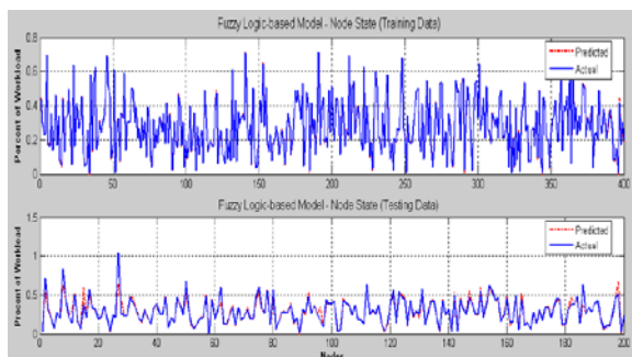
Figure 4. The fuzzy model – Node state (training and testing accuracy measures)
