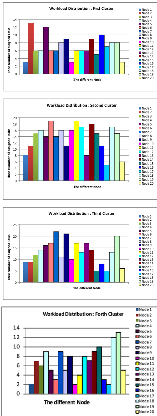
Figure 6. The workload of nodes in different clusters at a certain amount of time using random distribution algorithm (after assigning 800 tasks)
