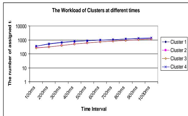
Figure 10. The clusters states at different times
