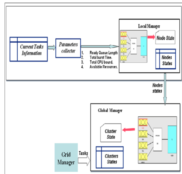
Figure 2. The architecture of the proposed scheme
