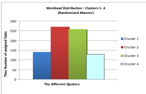
Figure 7. The workload distributed randomly among different clusters at a certain amount of time (after assigning 800 tasks).
