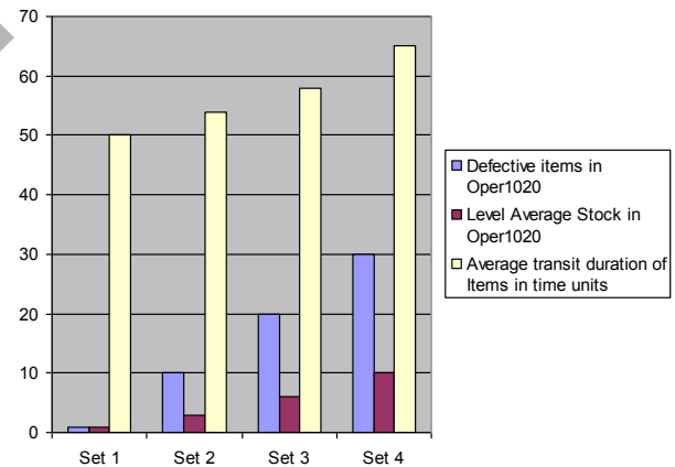
Figure 18. Simulation Results of coupled G-DEVS Route H80XX with LSIS_DME
