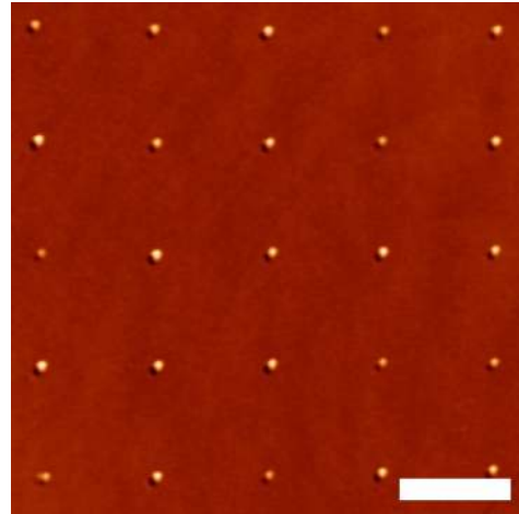
Figure 4 Atomic force micrograph of site-controlled QDs with 1 \mu\text{m} lattice period in a square lattice grown on a mesa structure. The scale bar represents 1 \mu\text{m} . Reprinted with permission from [93]. ©2008, AIP Publishing LLC.
