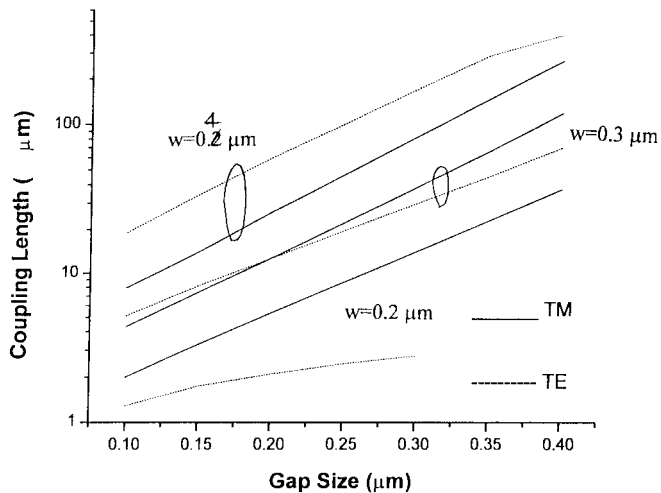
Fig. 3. Coupling length as a function of the gap size and the waveguide width ( w ), for both TE and TM polarizations.
