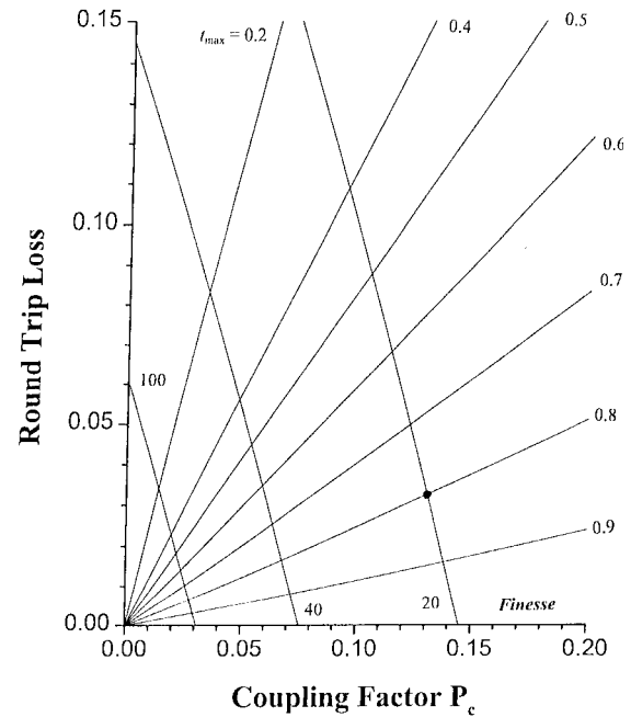
Fig. 4. Contour plots of constant finesse and constant t_{\text{max}} , as a function of the coupling factor P_c , and the round-trip loss L_{rt} . The solid dot represents the experimental data discussed in text.
