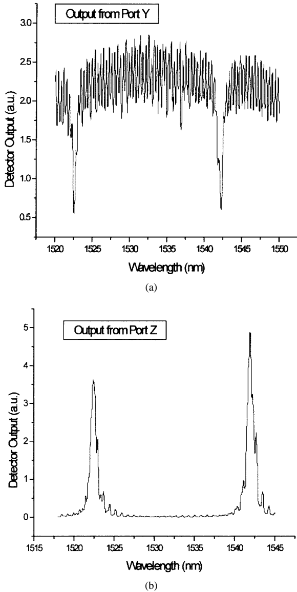
Fig. 2. The reflection and transmission spectra of a waveguide-coupled resonator with a cavity length of 31 \mu\text{m} , g = 0.2 \mu\text{m} and l = 6 \mu\text{m} , for the TM polarization.
