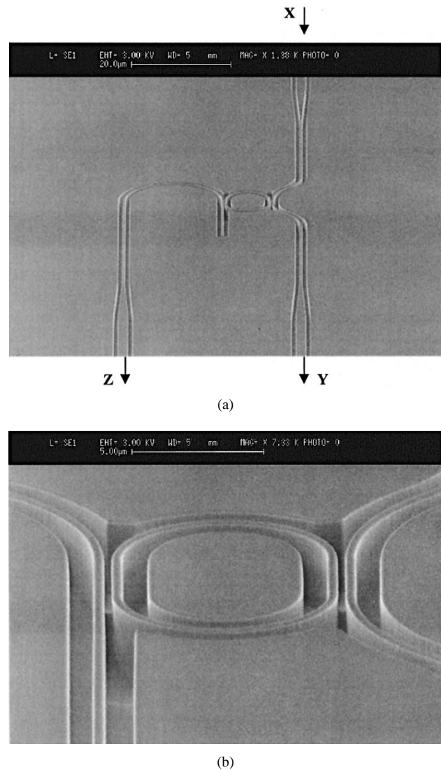
Fig. 1. Scanning-electron microscope images of (a) a resonator-based channel dropping filter and (b) the racetrack resonator.
