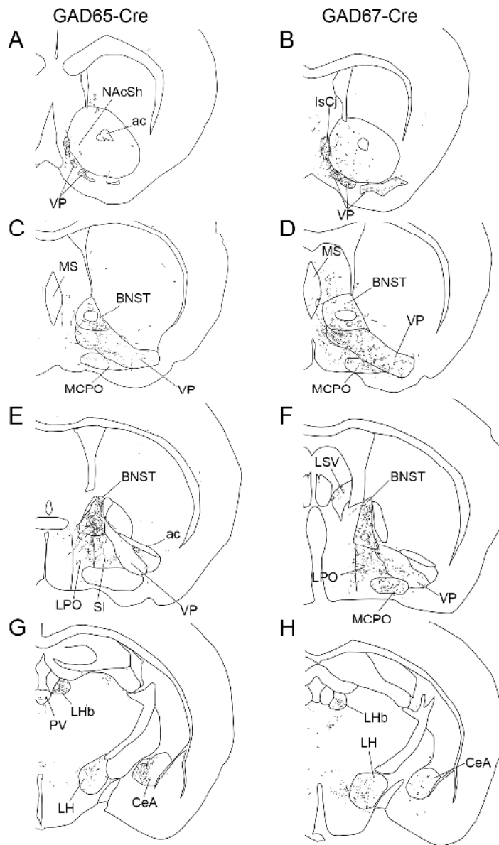
Figure 4. Coronal diagrams of line drawings of labeled fibers in representative cases from similar levels in both GAD65-IRES-Cre mice (Case S3; A, C, E, G, I, K, M, O) and GAD67-Cre mice (Case GC 153; B, D, F, H, J, L, N, P). 171x230mm (300 x 300 DPI)
