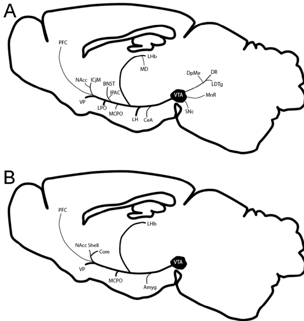
Figure 13. Summary diagram of ventral tegmental area GABAergic (Panel A) and glutamatergic (Panel B) efferents. The thickness of the arrows roughly depicts the density of the projection. 81x90mm (300 x 300 DPI)
