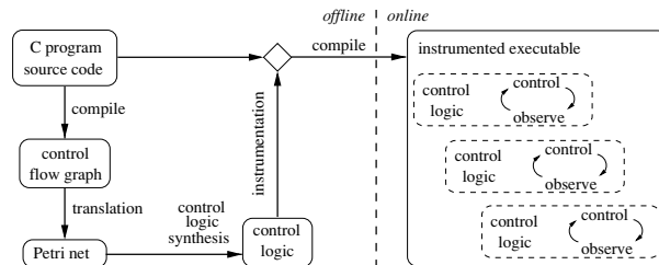
Figure 1: Gadara Architecture.
