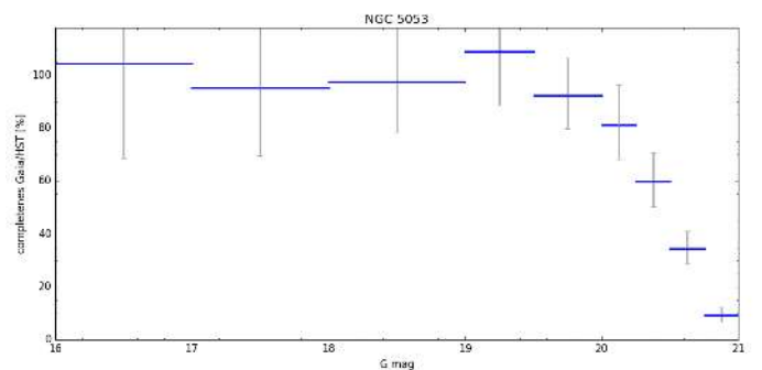
Fig. 14. Completeness of Gaia relative to HST in the area around NGC 5053 featuring stellar densities under 1 million per square degree.
