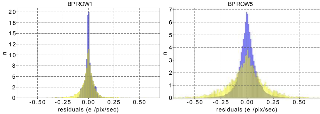
Fig. 9. Residual distribution (normalised to the same area) for the stray light maps. In blue the data obtained from 1D transits, in yellow from 2D transits. The left plot shows the best case (for BP ROW1 with scatter \sim 0.031 for 1D data and \sim 0.057 for 2D data), while the right plot shows the worst case (for BP ROW5, with scatter \sim 0.075 for 1D data and \sim 0.161 for 2D data).
