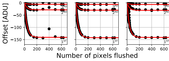
Fig. 3. Black dots in each panel show the excursion in bias level measured on-ground in an RVS test device for the first, second, and third pixels after the flush/read transition as a function of the number of flushes beforehand. Red lines show fitted analytical calibration functions for each of the three pixels. Each panel presents a different pattern of flushes. The saturation effect after a large number of flushes is evident, as is the rapid recovery in the subsequent read pixels after the first (each of the three red lines). The data shown in the panel on the left also show the perturbation resulting from a glitch after a pause in the serial readout (see text). Figure adapted from Boudreault & Cropper (2011a).
