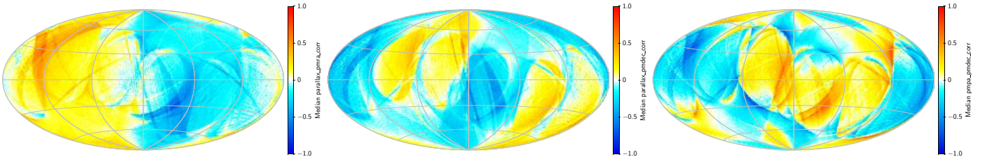
Fig. B.5. Correlation coefficients at G \approx 15 for sources with a five-parameter astrometric solution. Maps of the correlations at other magnitudes are very similar to these. Left : correlation between \varpi and \mu_{\alpha^*} . Middle : correlation between \varpi and \mu_{\delta} . Right : correlation between \mu_{\alpha^*} and \mu_{\delta} .
