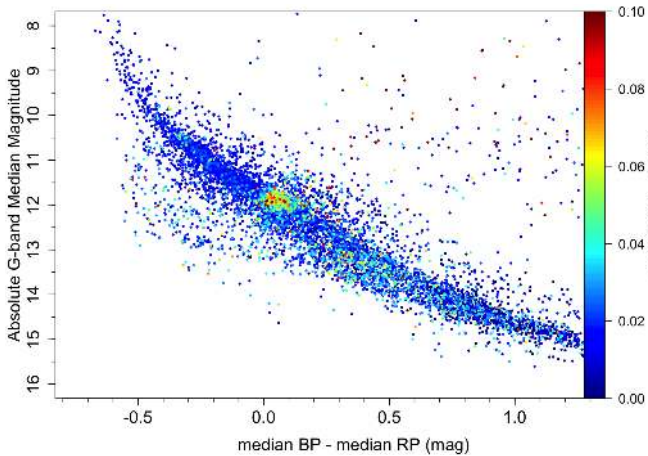
Fig. 10. Same as Fig. 9, but focusing on the white dwarf sequence and plotting all classified variables within 200 pc with a relative uncertainty for the parallax better than 5%. A close inspection of this sequence reveals amplitudes at the level of 40 mmag in various regions.
