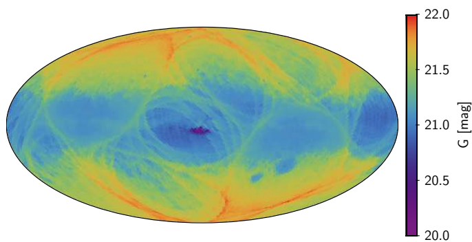
Fig. 2. Map in Galactic coordinates of the 99th percentile of the G magnitude at healpix level 5, i.e. in 3.36 \square^\circ pixels.
