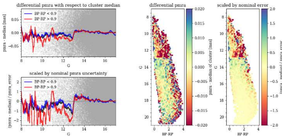
Fig. 25. Same as Fig.24, but for \mu_{\alpha^*} .
