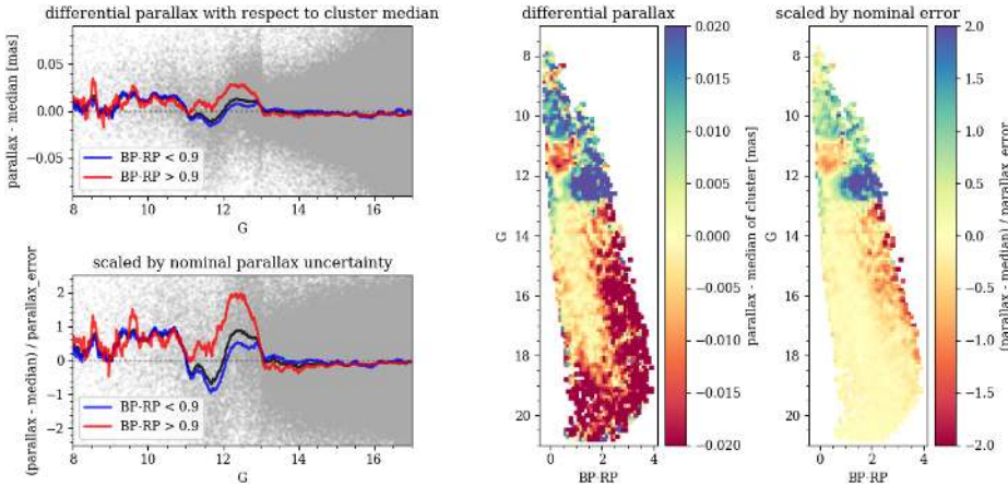
Fig. 17. Left: \Delta_{\sigma} (top) and scaled to the nominal uncertainties \Delta_{\sigma} (bottom) versus G for the whole sample of clusters. The solid lines show the LOWESS (locally weighted scatterplot smoothing) of the stars bluer (redder) than G_{BP} - G_{RP} = 0.9 (blue and red lines), while the black line is for the whole sample. Right: CMD of the whole sample where the colour shows the differential parallax to the median.
