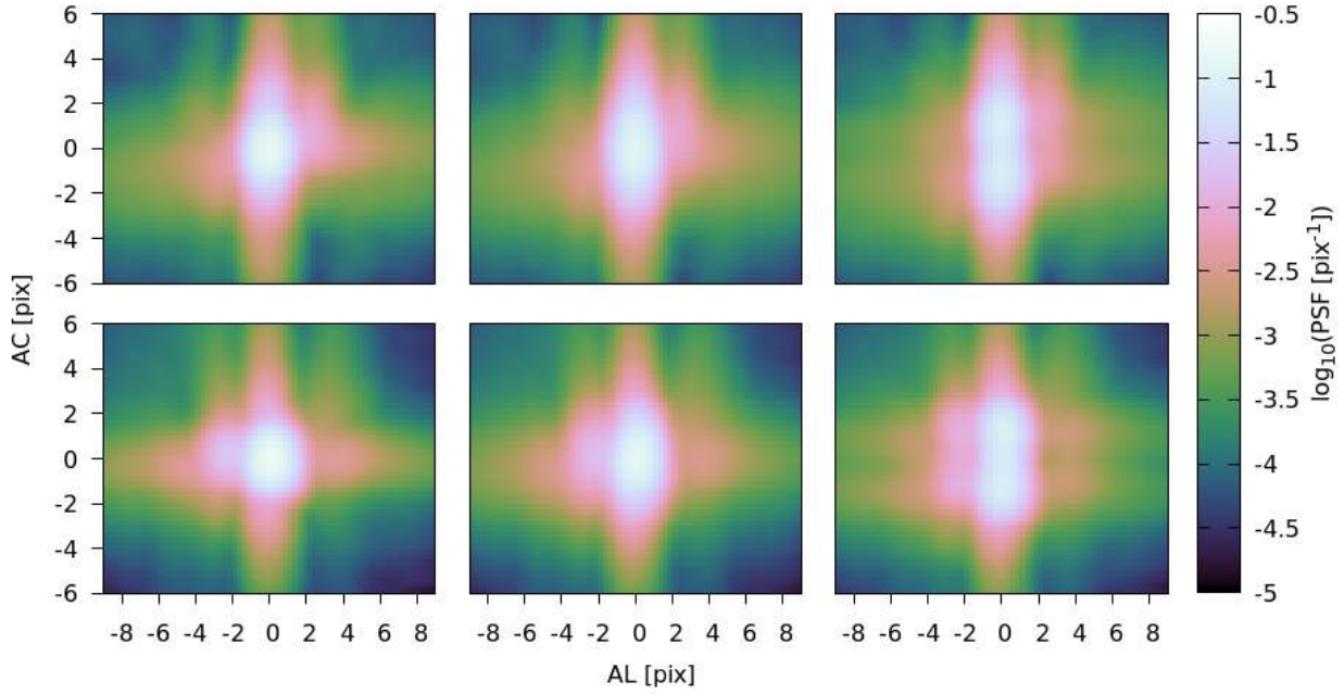
Fig. 13. AC rate ( \mu ) variation for the FOV1 ( top row ) and FOV2 ( bottom row ) calibrations for CCD row 4, strip AF5, gate 0. The plots correspond to AC rate values of 0.0 ( left ), 0.6 ( middle ), and 1.0 ( right ) pixels per second. See the text for details.
