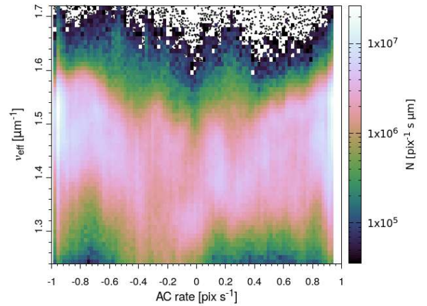
Fig. 6. Distribution in the (\dot{\mu}, v_{\text{eff}}) plane of the observations depicted in Fig. 5. There is a correlation between \dot{\mu} and v_{\text{eff}} that evolves over time (see text).
