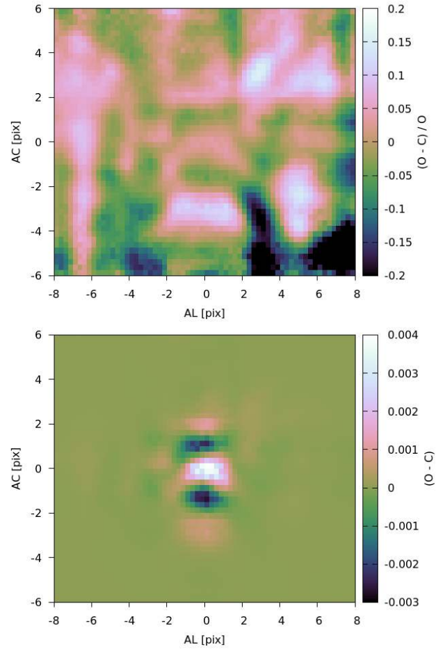
Fig. 16. Median relative ( top ) and absolute ( bottom ) residuals about the model for a selection of 2D observations used in the PSF calibration. Observations are selected from one calibration unit over a ten revolution period, and span the magnitude range 12 \lesssim G \lesssim 13 .
