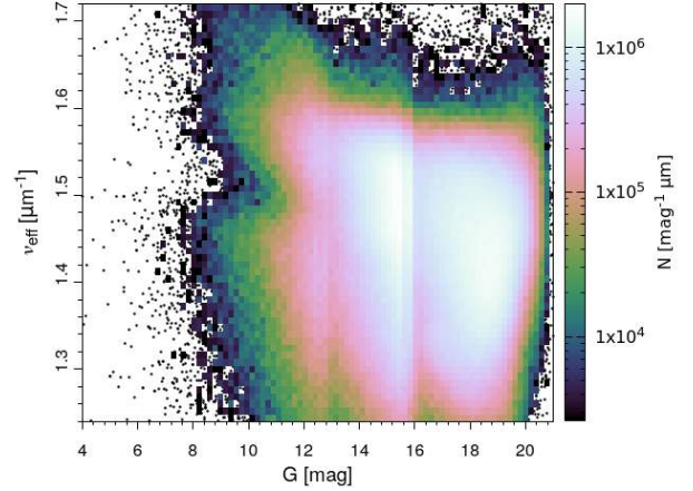
Fig. 5. Distribution in the (G, v_{\text{eff}}) plane of 1 604 769 eligible observations that have passed the first stage of selection.
