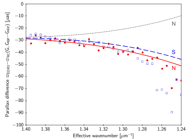
Fig. C.3. Differential parallax bias estimated by means of RC stars. The points show the locations of the ridges in Fig. C.2 for area N (filled red circles) and S (open blue squares). The curves show the expected locations at G = 17 according to Table 6 for area N (solid red) and S (long-dashed blue), assuming that the curvature with colour ( j = 2 ) is the same in both areas. If the curvature had flipped sign with \beta , the ridge location for area N should instead follow the up-bending, short-dashed black curve.
