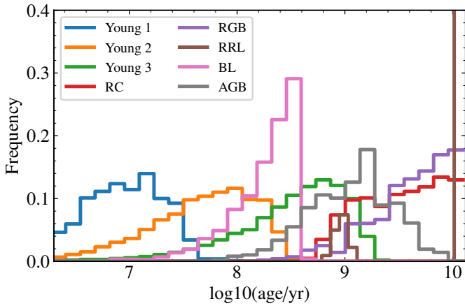
Fig. 3. Estimated age distribution of the selected evolutionary phase. Based on a simulation using a constant star formation rate, the age-metallicity relation by Harris & Zaritsky (2009) , and PARSEC1.2 models
