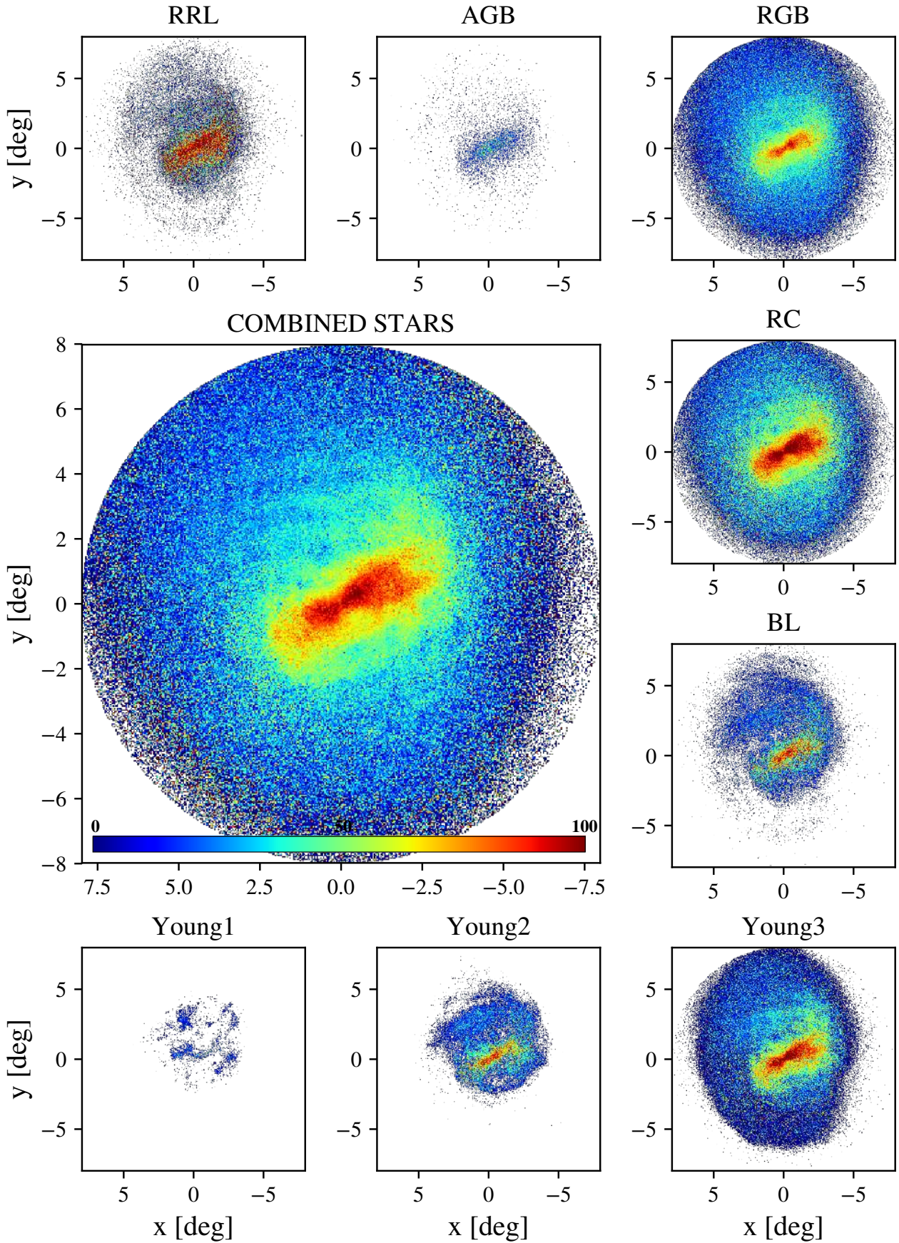
Fig. B.3. Azimuthal velocity dispersion maps \sigma_\phi of the LMC for the combined sample ( main panel ) and the various evolutionary phases. The linear velocity scale shown by the colour bar in the main panel is the same in all subpanels and has been chosen to highlight velocity patterns better.
