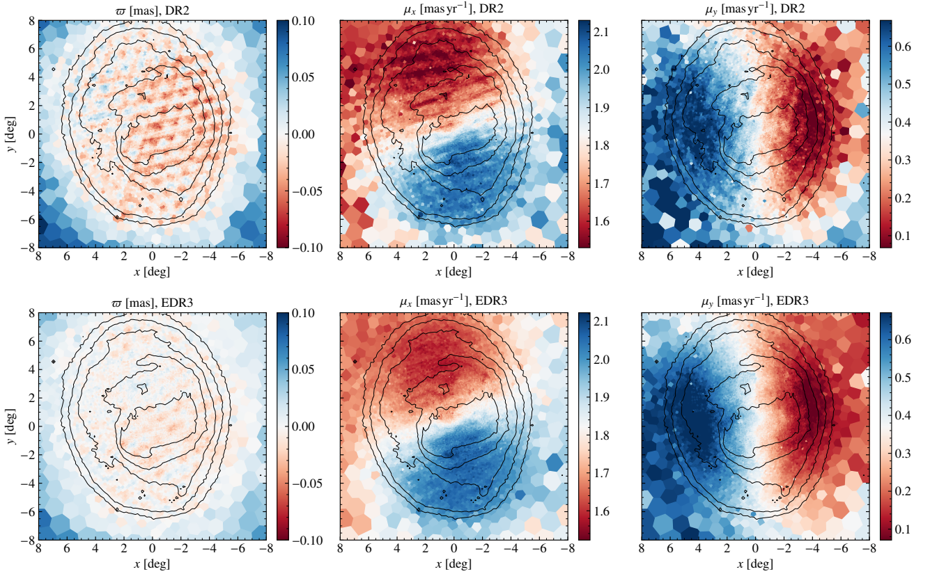
Fig. 4. Comparison of the parallaxes ( left ) and proper motions in the x and y directions ( middle and right , respectively) of LMC sources in Gaia DR2 ( upper panels ) and Gaia EDR3 ( lower panels ).
