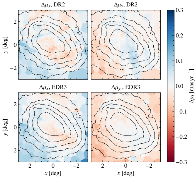
Fig. 7. Same as in Fig. 6, but for the SMC.
