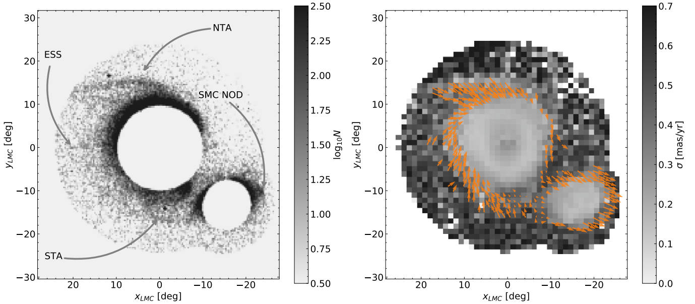
Fig. 17. Number count map for the LMCout sample ( left ): the names of the most notable substructures are given and, for a better visualisation, the inner parts of the LMC and SMC were omitted. Total velocity dispersion map ( right ): the velocity vector field is shown as orange arrows.
