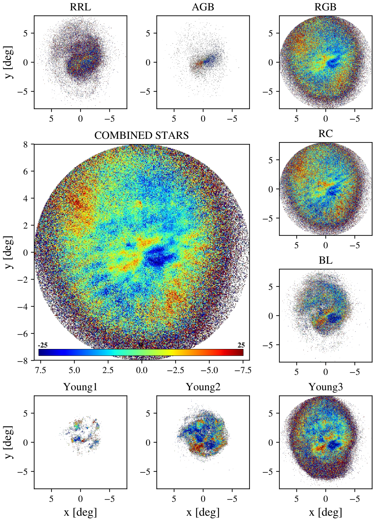
Fig. B.2. Radial velocity maps v_R of the LMC for the combined sample ( main panel ) and the various evolutionary phases. The linear velocity scale shown by the colour bar in the main panel is the same in all subpanels and has been chosen to highlight velocity patterns better.
