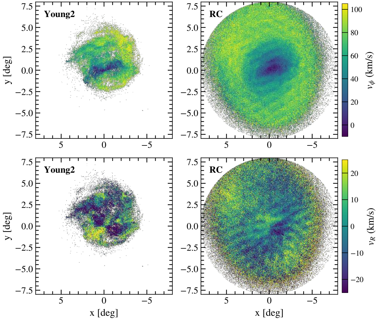
Fig. 12. Example of velocity maps for the LMC. Left and right columns: young and evolved evolutionary phases (Young 2 and RC, respectively, see Sect. 2.3). Upper and bottom rows: v_\phi and v_R , respectively. The linear velocity scales shown by colour bars are the same for the two stellar evolutionary phases and were chosen to show the structure inside the velocity fields more clearly.
