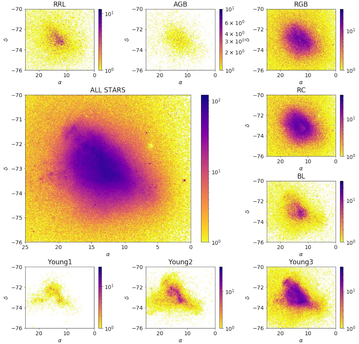
Fig. A.7. Sky density plots for the complete SMC clean sample and the different evolutionary phase subsamples.
