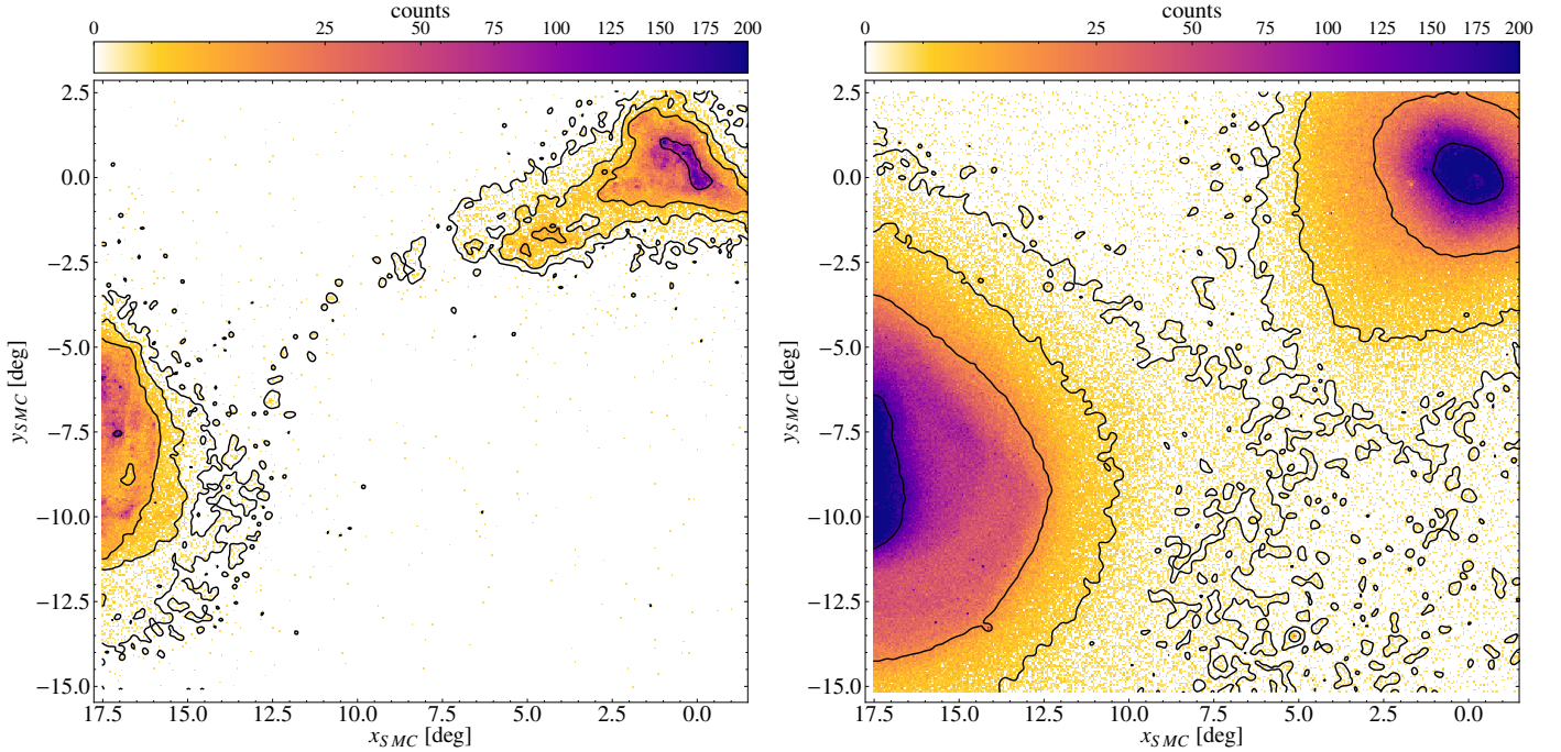
Fig. 15. Sky density plot for the Bridge region using the Young 1 and Young 2 evolutionary phases ( left panel ) and the RC evolutionary phase ( right panel ). The bin size is 0.06 deg in x and y . The colour bar is in log scale and the black contours are at the levels 0.1, 1, 5, and 70 (young evolutionary phases) and 0.25, 1.5, 15, and 165 (RC sample).
