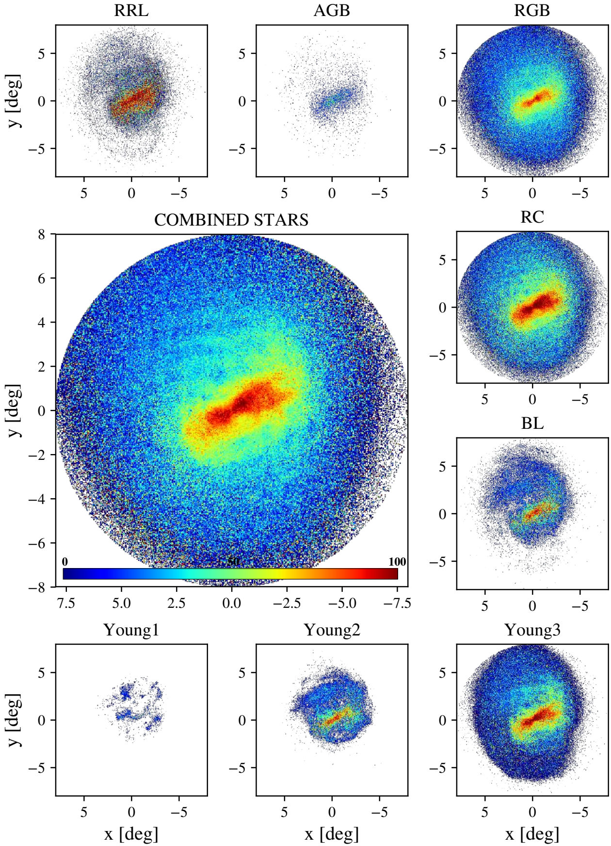
Fig. B.3. Azimuthal velocity dispersion maps \sigma_\phi of the LMC for the combined sample ( main panel ) and the various evolutionary phases. The linear velocity scale shown by the colour bar in the main panel is the same in all subpanels and has been chosen to highlight velocity patterns better.
