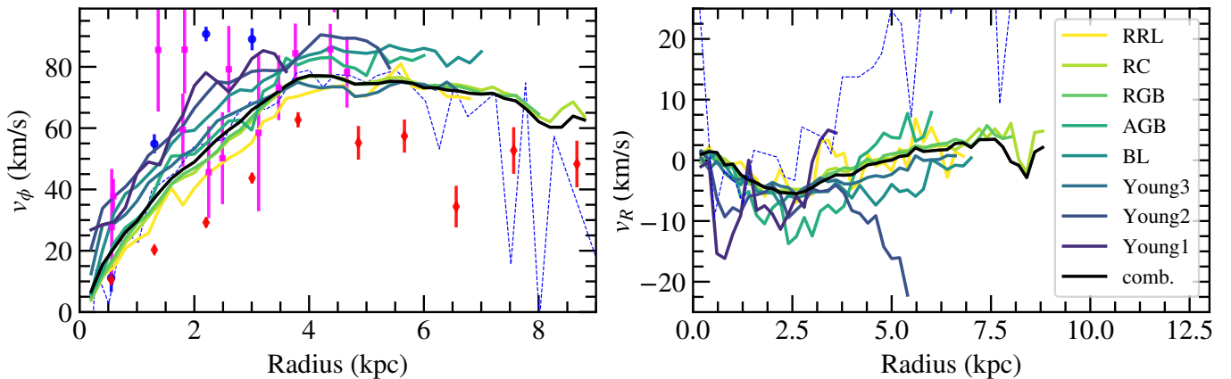
Fig. 14. Stellar velocity curves of the LMC. Left and right panels: rotation curves and radial motions, respectively. Coloured lines are for the eight evolutionary phases and the combined sample, as given by the legend. In the left panel, blue circles, red diamonds and magenta squares are the rotation velocities for the samples of younger and older stars from line-of-sight spectroscopic and HST astrometric measurements published in van der Marel & Kallivayalil (2014) . The dashed blue lines are the tangential and radial velocity profiles derived by Wan et al. (2020) from Gaia DR2 astrometry.
