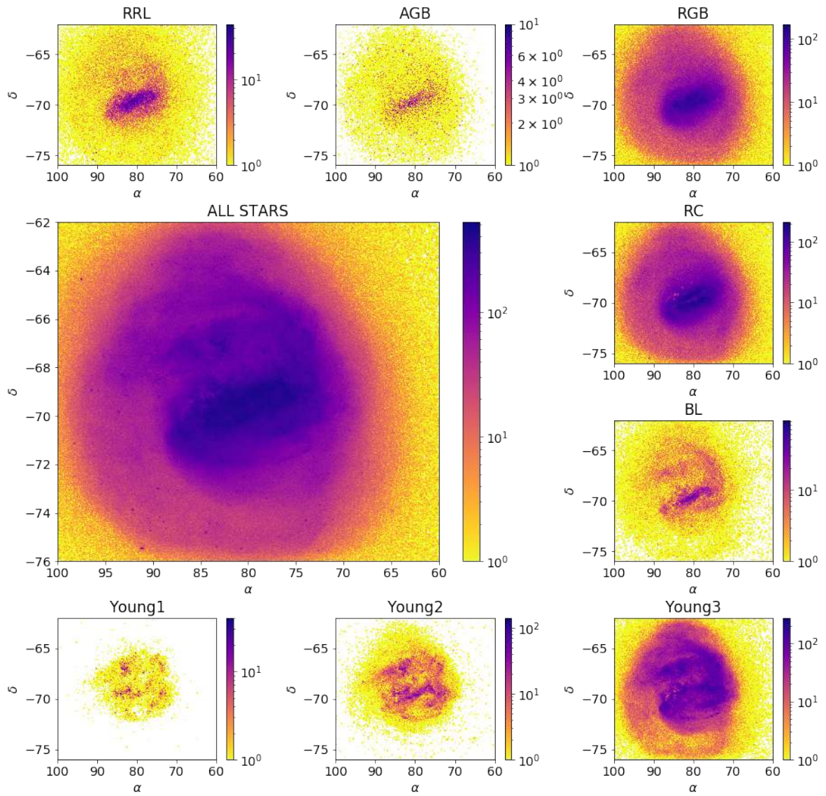
Fig. A.6. Sky density plots for the complete LMC clean sample and the different evolutionary phase subsamples.
