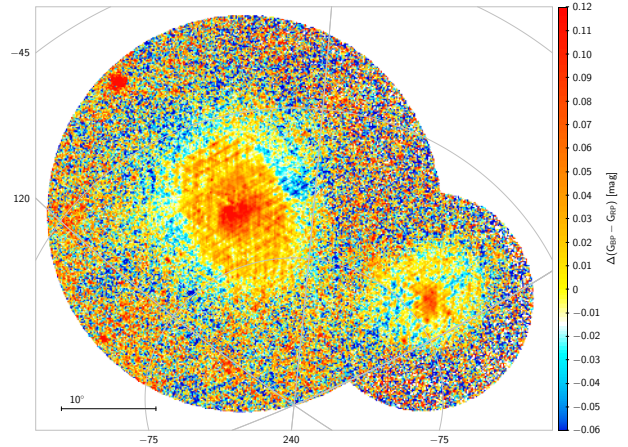
Fig. A.4. Mean change in colour, G_{BP} - G_{RP} , in Gaia DR2 and Gaia EDR3 for sources in the LMC and SMC. Positive values mean that the sources are now redder.
