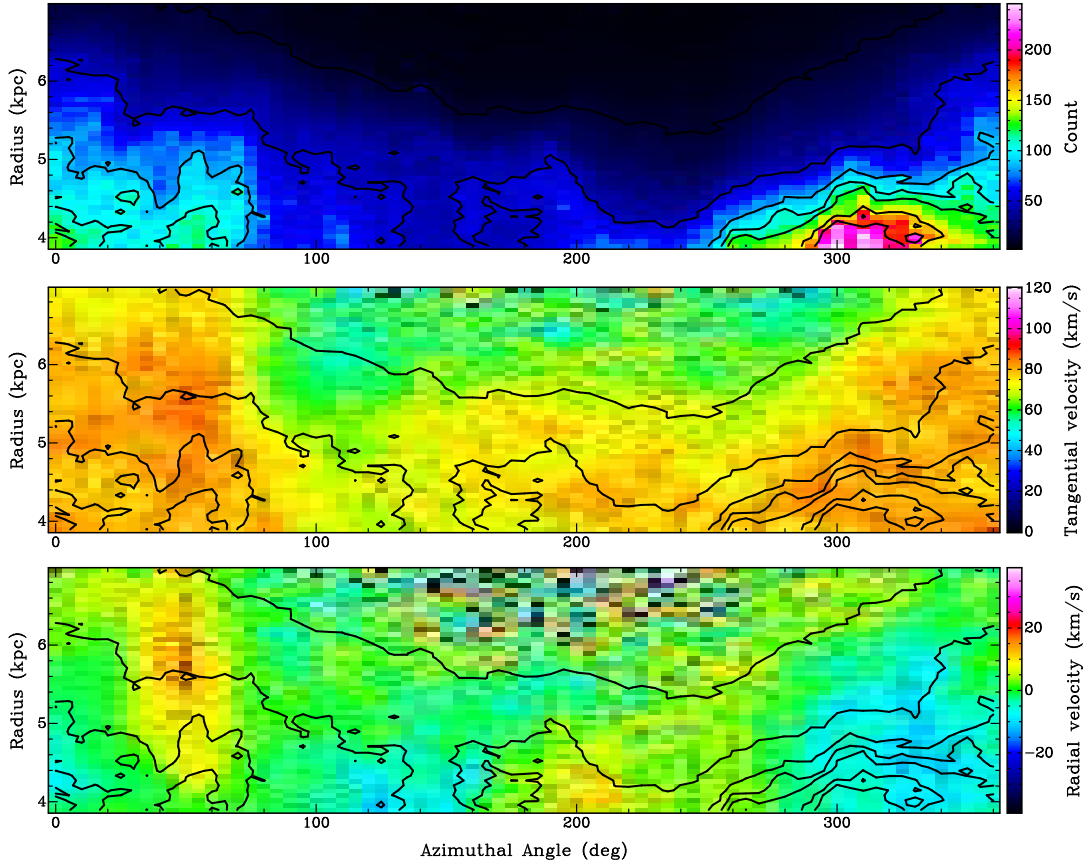
Fig. 21. Streaming motions across and along the eastern spiral arm of the LMC. The azimuth-radius diagrams show the stellar density ( top panel ), the tangential velocity ( middle panel ), and radial velocity ( bottom panel ). Contours represent the stellar density shown in the upper panel .
