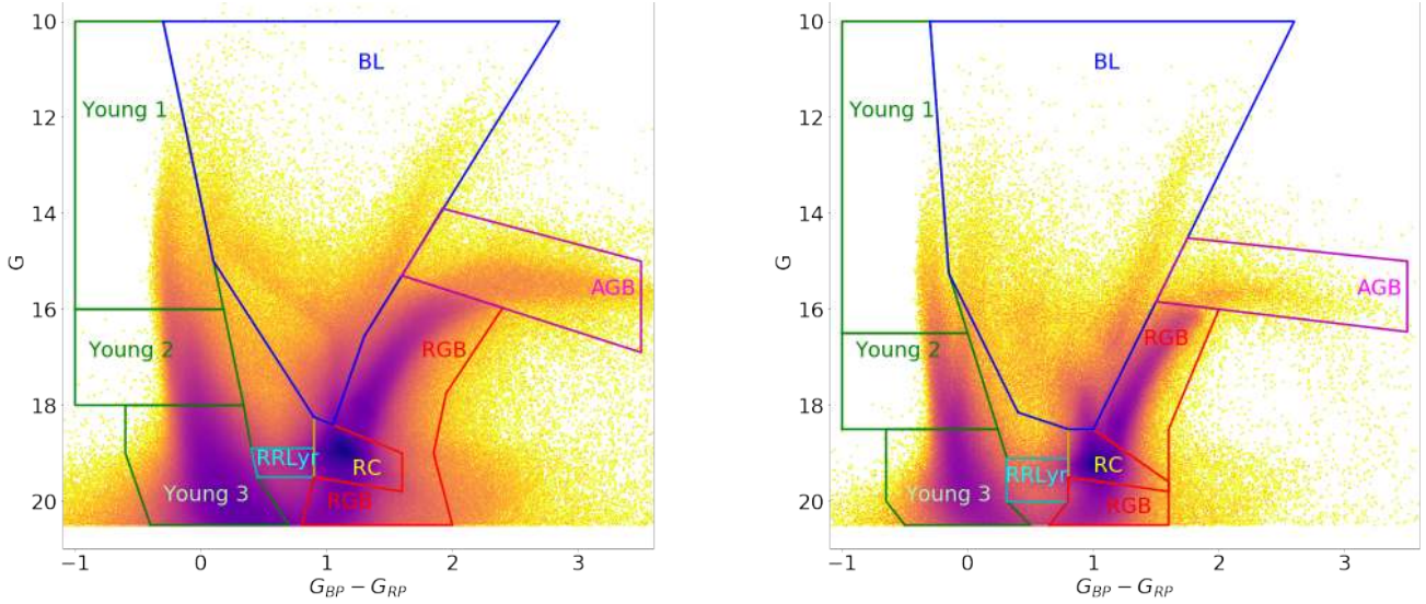
Fig. 2. Areas (as defined by the polygons given in the text) of the CMD for the LMC ( left ) and SMC ( right ) evolutionary phases. The colours are not corrected for reddening for the selection.
