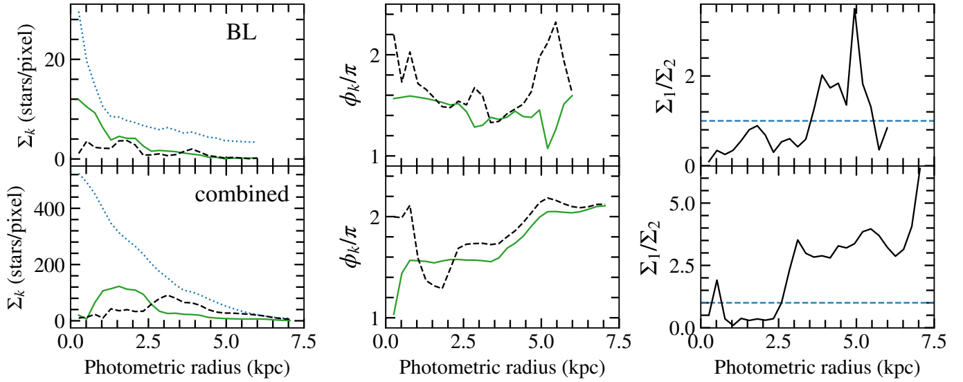
Fig. 19. Results of the Fourier transform of stellar density maps of the LMC for the BL and the combined samples ( upper and bottom panels , respectively). Left and middle panels : amplitude and phases of the first- and second-order asymmetries (dashed black and solid green lines, respectively). The axisymmetric density is shown as a dotted blue line. Right panel : k=1 perturbation over the bisymmetry strength ratio. The galactocentric radius is given here in the photometric frame, with \Omega_{\text{phot}} = 10^\circ as the reference photometric position angle.
