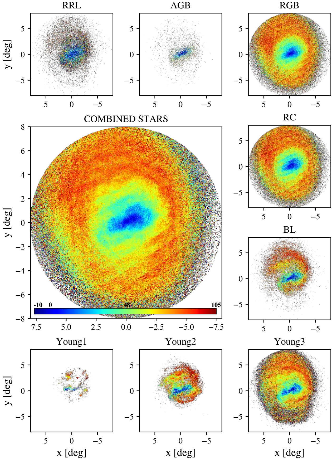
Fig. B.1. Azimuthal velocity maps v_\phi of the LMC for the combined sample ( main panel ) and the various evolutionary phases. The linear velocity scale shown by the colour bar in the main panel is the same in all subpanels and has been chosen to highlight velocity patterns better.
