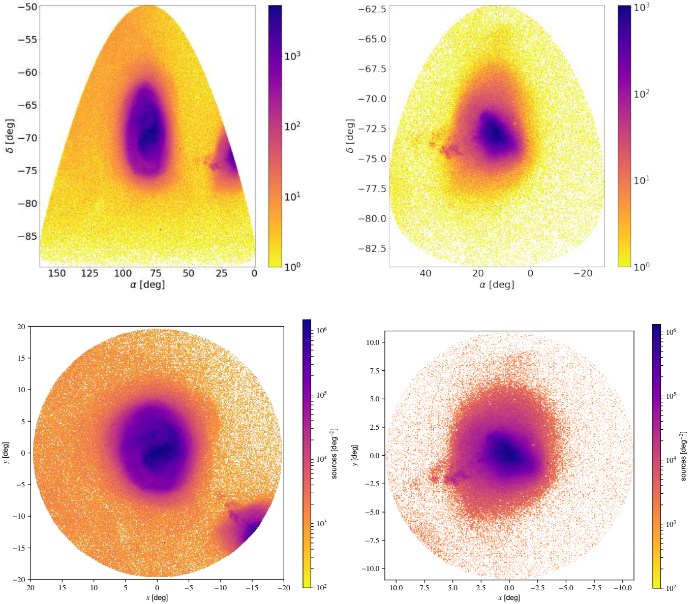
Fig. 1. Sky density plots for the LMC ( left ) and SMC ( right ) clean samples (after spatial and proper motion selection). Top row: plots in equatorial coordinates. Bottom row: orthographic projection (as used in Sect. 3)
