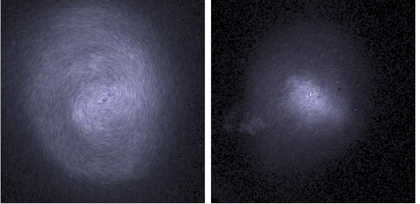
Fig. 8. Illustration of the proper motion field of the LMC ( left ) and SMC ( right ) using line-integral convolution. We set the alpha parameter (opacity) of the coloured lines according to the density, with the densest regions being the most opaque.
