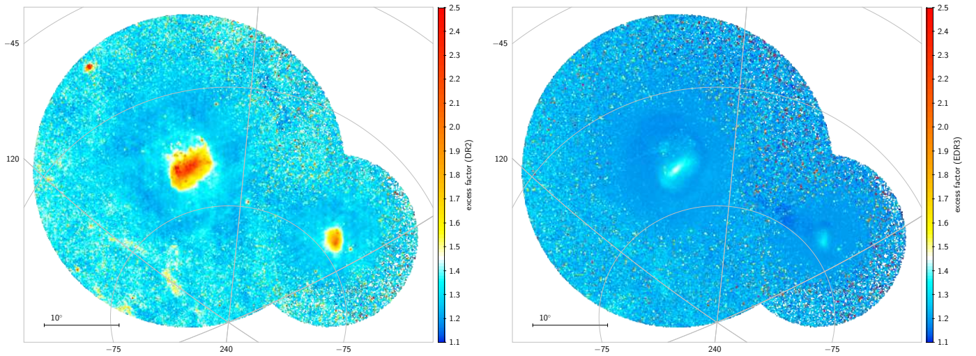
Fig. 9. Photometric excess factor, i.e. the sum of fluxes in the G_{BP} and G_{RP} bands over the G flux. Left: for Gaia DR2. Right: for Gaia EDR3.
