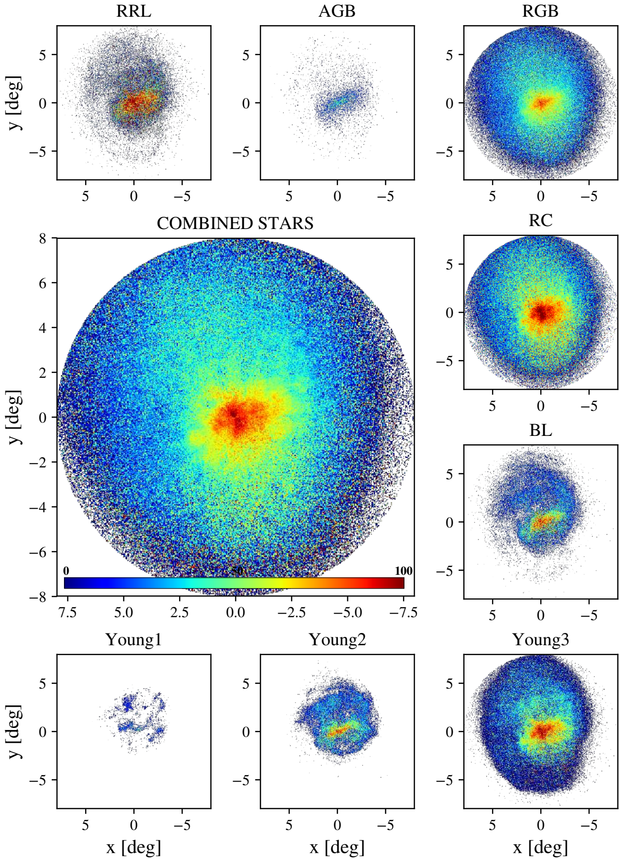
Fig. B.4. Radial velocity dispersion maps \sigma_R of the LMC for the combined sample ( main panel ) and the various evolutionary phases. The linear velocity scale shown by the colour bar in the main panel is the same in all subpanels and has been chosen to highlight velocity patterns better.
