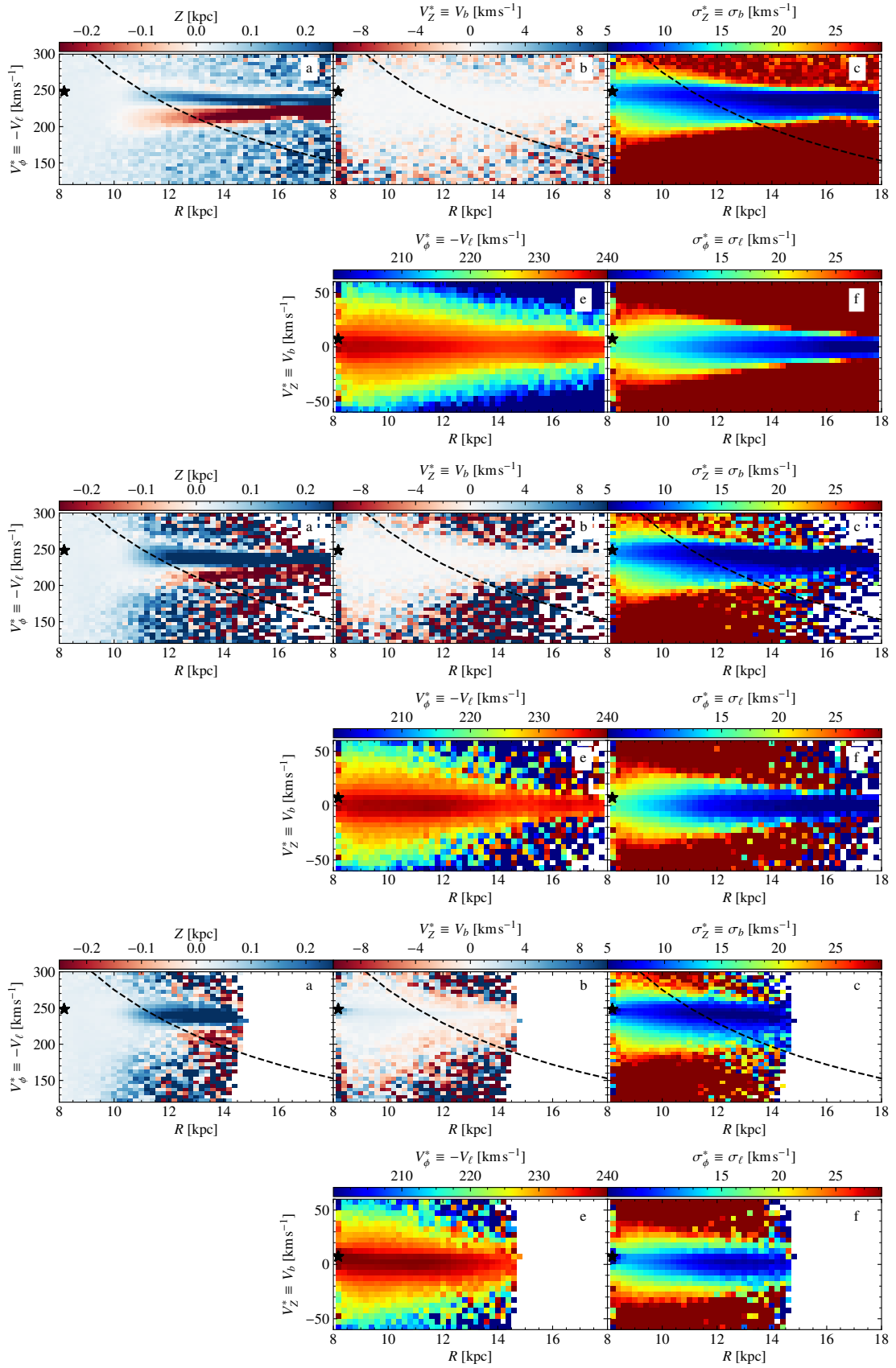
Fig. E.6. Phase space projections for model and mock data. Same as Fig. 14 but for the UM ( top ), the UM with the sources that in GOG have \varpi/\sigma_\varpi > 3 ( middle ), and for GOG with the selection \varpi/\sigma_\varpi > 3 ( bottom ). The phase space spiral does not exist in GOG and panels d are not shown.
