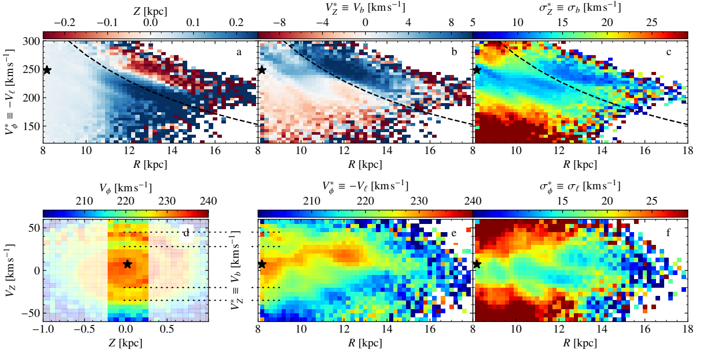
Fig. 14. Phase space projections of the Galaxy disc. The plots show for the AC20- w/\sigma_w > 3 sample: (a) median Z coordinate in the R - V_\phi^* plane; (b) median vertical velocity V_z^* in the same projection; (c) dispersion in the V_z^* velocity in the same projection (computed as the 1.5MAD); (d) phase spiral in the 6dsample in EDR3 for stars in the Galactic radial range |R - R_0| < 0.2 kpc; (e) median azimuthal velocity V_\phi^* in the R - V_z^* plane; (f) dispersion in V_\phi^* in the same plane. The bimodality appears in the outer parts of the disc in panels a–c , with the separation marked with a line of constant angular momentum L_z^* = 2750 \text{ km s}^{-1} \text{ kpc} . Panel e : evolution of a slice of the phase spiral (marked in brighter colours in panel d ) is seen for smaller radii, while a signature related to the above bimodality is seen beyond \sim 12 kpc in panels e and f .
