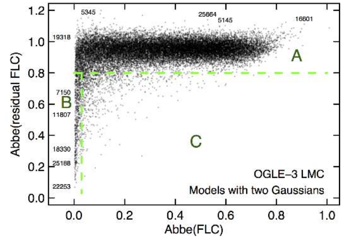
Fig. 15. Abbe value \mathcal{A}_{\text{resFLC}} of the residual folded light curves versus Abbe value \mathcal{A}_{\text{FLC}} of the folded light curve of OGLE-III eclipsing binaries in the LMC, for all models containing two Gaussians (with or without ellipsoidal component). The dashed horizontal and vertical green lines delimit the three regions A, B and C mentioned in the text. Sources labeled in the figure have their folded light curves shown in Figs. 16 to 17.
