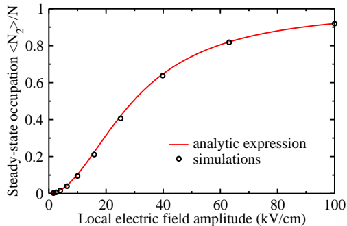
Figure 4. Comparison between simulation results (black circles) and the analytic expression (3.9) for the normalized steady-state occupation density of the upper emission state \langle N_2 \rangle / N of the four-level system (red solid line) when pumping at the absorption resonance \lambda_{0,a} = 680 nm. The parameters of the four-level gain material are given in table 2 and correspond to a saturation field amplitude of E_{\text{sat}} \approx 29.4 kV/cm. (Online version in colour.)
