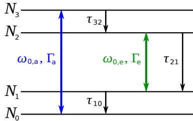
Figure 2. Sketch of the four-level system and its parameters. (Online version in colour.)
