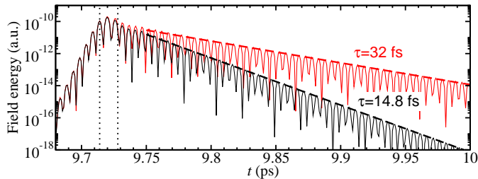
Figure 10. Temporal decay of electromagnetic energy inside the double-fishnet resonator for the case without pumping (black) and for full loss compensation (red). The vertical dotted lines indicate the FWHM of the probe pulse. (Online version in colour.)
