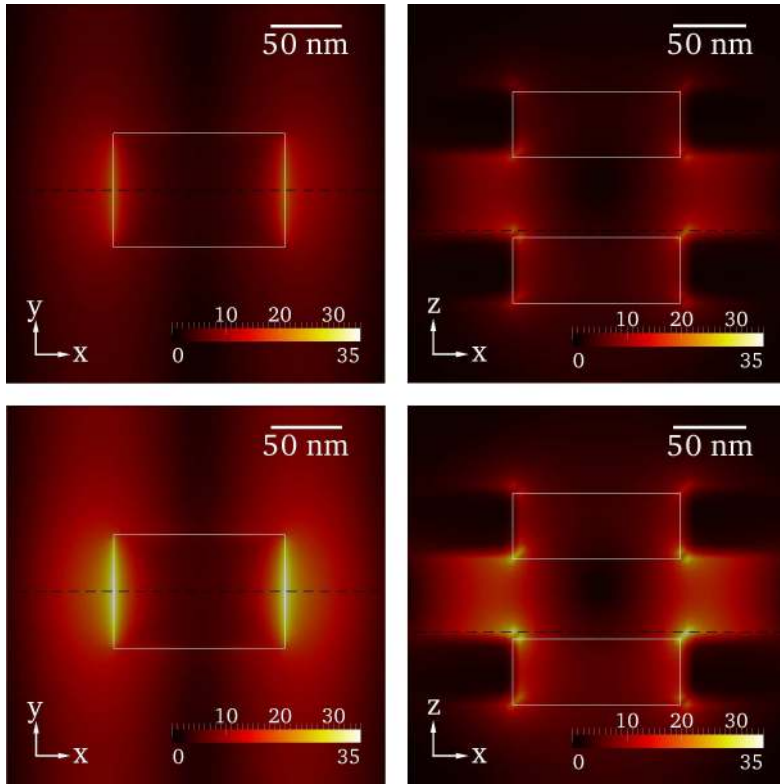
Figure 8. Electric field enhancement in two perpendicular planes of the unit cell at the probe wavelength without pumping (upper row) and with full loss compensation (lower row). This confirms that the spatial structure is retained while the amplitude is enhanced. The white rectangles highlight the position of the holes and the black dashed lines show the intersection of the two planes in each row. (Online version in colour.)
