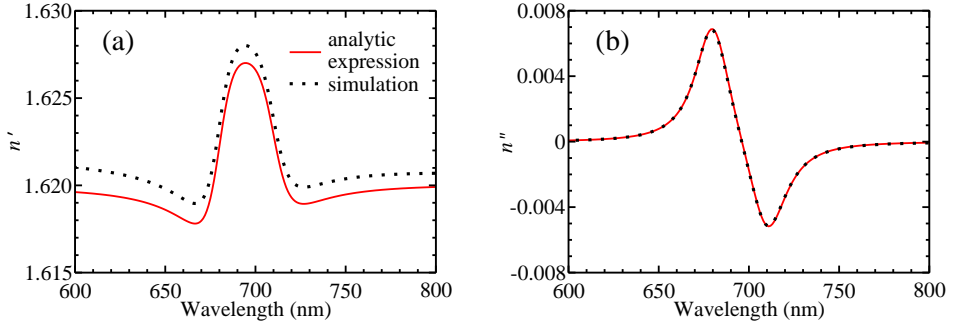
Figure 3. Comparison between numerical simulations (black dotted line) and the analytic equations (3.4) (red solid line) for the real (a) and imaginary (b) part of the refractive index of a thin slab of gain material with \Delta N_a = -N_0 = -N/2 and \Delta N_e = N_2 = N/2 . The parameters of the four-level gain material are given in table 2 and the host refractive index is n_h = 1.62 . (Online version in colour.)
