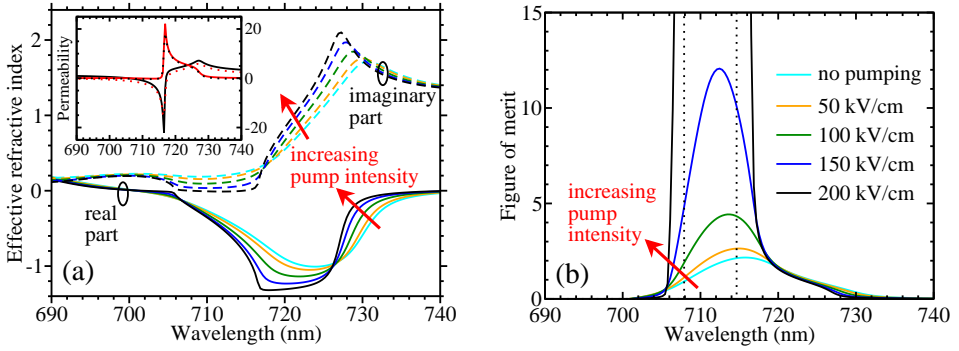
Figure 11. (a) Real and imaginary part of the retrieved effective refractive indices of the double-fishnet structure for different pump amplitudes. The peak electric field amplitude of the pump increases in steps of 50 kV/cm from no pumping (cyan line, lightest) to a maximum of 200 kV/cm (black line, darkest). The inset shows the real and imaginary parts of the effective permeability (black and red line, respectively) and the result of the Kramers-Kronig relation (black and red dotted lines) for the highest peak electric field amplitude of 200 kV/cm. (b) The figures of merit (FOMs) for the same pumping amplitudes. The vertical dotted lines indicate the exact wavelengths at which the FOM diverges. (Online version in colour.)
