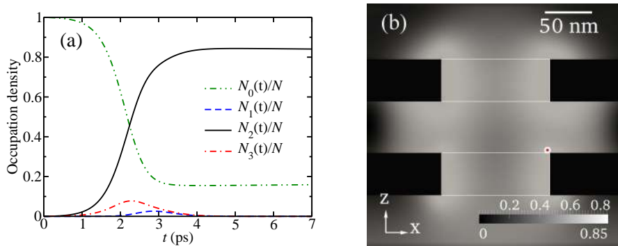
Figure 5. (a) Time dependence of the occupation densities of the gain medium recorded at a position of high inversion given by a red dot in (b). (b) Snapshot of the occupation inversion after the pump process in a plane inside the double-fishnet unit cell. The white rectangular outlines highlight the positions of the holes and the rectangular black areas are the silver films. (Online version in colour.)
