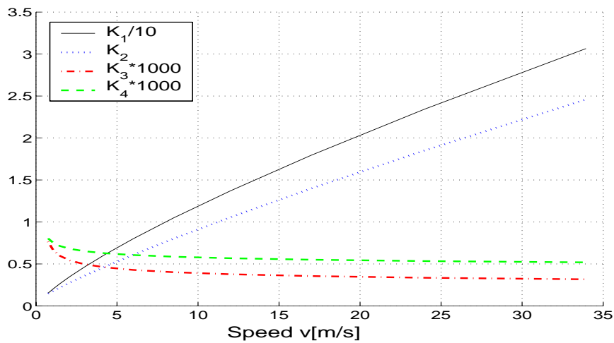
Fig. 6. Gain K(v) , as a function of v .
