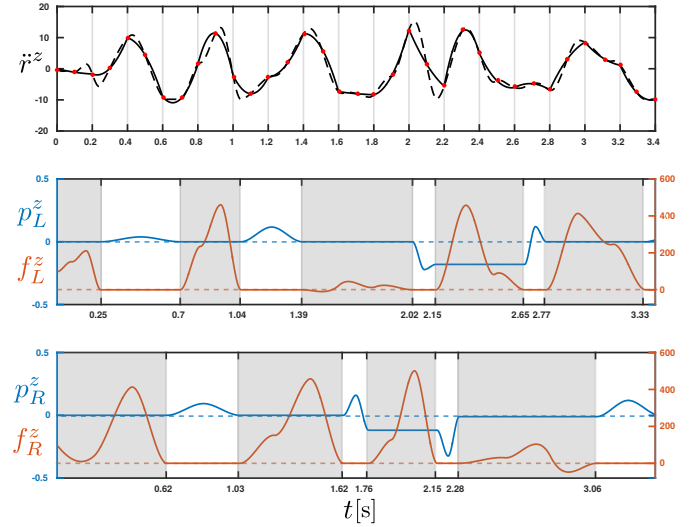
Fig. 6. A generated motion plan for a 20 kg-bipedal robot crossing a 1 m wide gap (see video at 01:09). The plots show the base vertical acceleration \ddot{r}^z(t) as well as the vertical position and vertical force of the left (L) and right (R) leg. The planned base vertical acceleration is compared to the vertical body acceleration that results from evaluating (2) with the current footholds and forces. In this example we use fourth-order polynomials of duration 0.2 s for the base motion parameterization. The red nodes, spaced 0.1 s apart, show the times at which the dynamic constraint is enforced in the NLP. We use two third-order polynomials to parameterize each foot motion in swing-phase (white area), and three third-order polynomials for each force profile per foot in stance-phase (shaded area).
