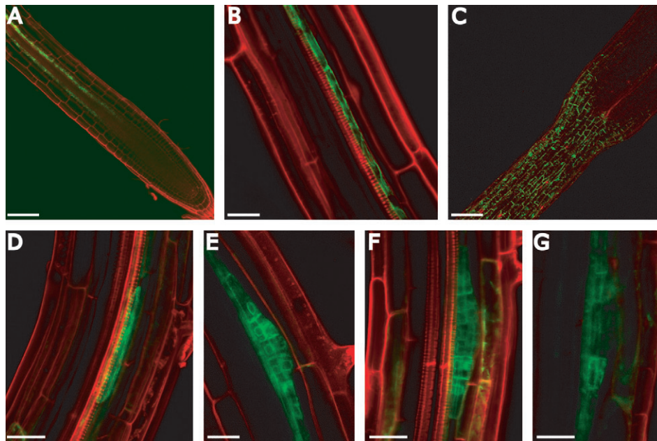
Fig. 1. GFP expression in the enhancer trap lines J0121 (A–C) and J0192 (D–G). (A, B, D, E, F, G) Longitudinal confocal sections of roots and (C) projected confocal view of the top part of a hypocotyl of living plants showing GFP fluorescence (green) and counterstained with propidium iodide (red). (A) GFP expression starts in the pericycle cells of the elongation zone. No GFP fluorescence is visible in the root meristem. (B) Expression in pericycle cells adjacent to a xylem strand. (C) Expression in the hypocotyl epidermis. (D) Expression in a stage I primordium. (E) Expression in a stage II primordium. (F) Expression in a stage III primordium. (G) Expression in a stage V primordium. Stages are defined according to Malamy and Benfey (1997).
