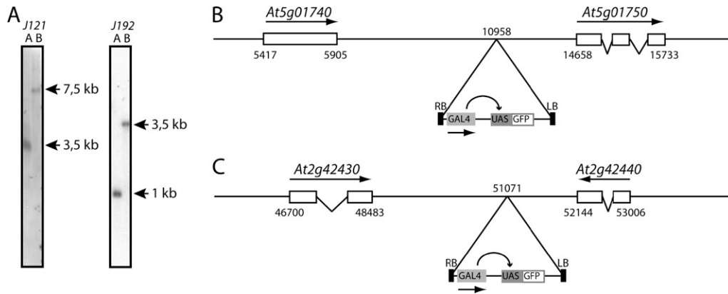
Fig. 3. Molecular characterization of the enhancer trap lines J0121 and J0192. (A) Southern blot hybridization of genomic DNA isolated from J0121 and J0192 plants. 3 \mu g of genomic DNA was digested with ApoI and BglII and hybridized with a ^{32} P-labelled GAL4 probe. (B) Enhancer trap T-DNA insertion site in J0121. Positions are relative to BAC clone T20L15. (C) Enhancer trap T-DNA insertion site in J0192. Positions are relative to BAC clone MHK10.
