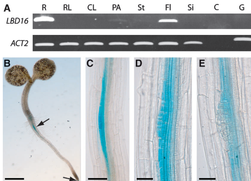
Fig. 4. LBD16 expression pattern. (A) RT-PCR analysis of LBD16 expression in 10-d-old root tissues (R), rosette leaves (RL), cauline leaves (CL), 10-d-old shoot apex (PA), inflorescence stem (St), flowers (Fl), and siliques (Si). A control without cDNA (C) and a genomic DNA control (G) were also included. LBD16 primers are situated on both sides of an intron so that the genomic DNA amplification is 749 bp bigger than the cDNA amplification product. Amplification of the constitutive ACTIN2 gene was used as a positive control. (B) 3-d-old LBD16-GUS Arabidopsis seedling showing blue GUS staining in the columella at the root tip and in a lateral root primordium (arrows). (C) GUS activity in a stage I lateral root primordium from a 5-d-old LBD16-GUS plant. (D) GUS staining in a stage III LRP from a 7-d-old LBD16-GUS seedling. (E) GUS activity in a stage IV LRP from a 7-d-old LBD16-GUS plant. Bars are 0.5 mm (B), 50 \mu m (C), and 25 \mu m (D, E).
