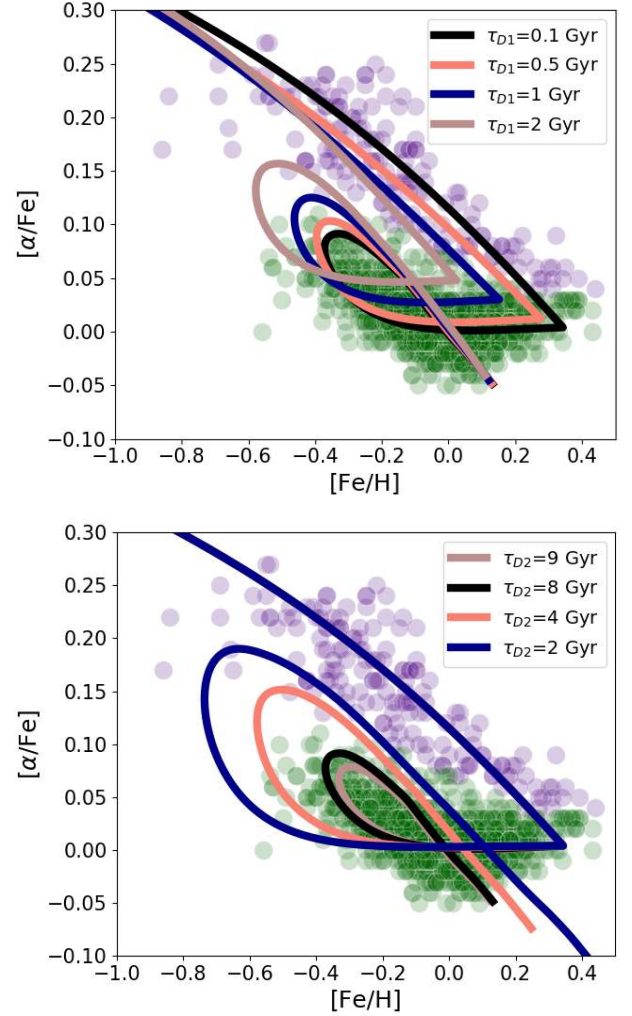
Fig. 13. Effects on the chemical evolution of the solar neighbourhood in the [\alpha/\text{Fe}] versus [\text{Fe}/\text{H}] plane of different timescales for primordial gas infall. Upper panel: timescale variations for primordial gas accretion related to the high- \alpha sequence ( \tau_{D1} ). Lower panel: timescale variations for primordial gas accretion related to the low- \alpha sequence ( \tau_{D2} ).
