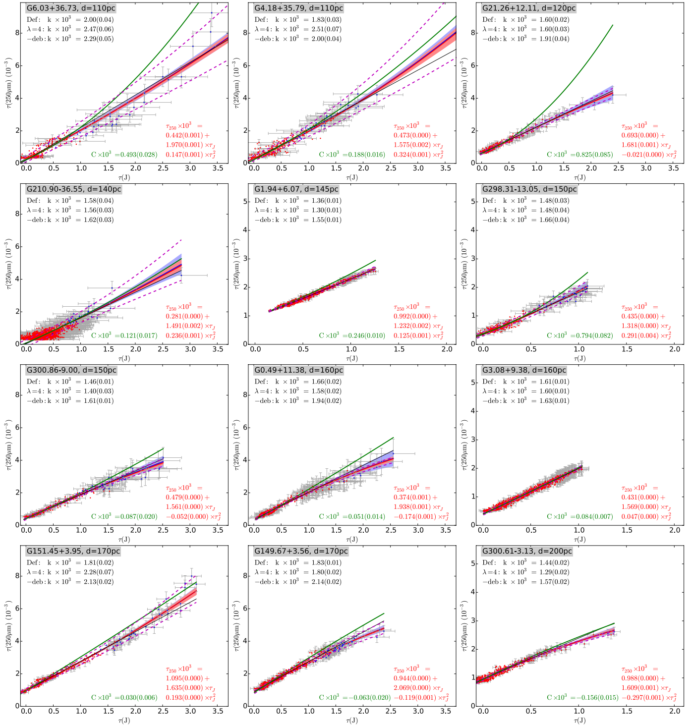
Fig. 8. Fits of \tau(250 \mu\text{m}) vs. \tau(J) in selected fields ordered by increasing distance. The red and blue points (dust temperature above and below 14 K) with error bars are the bias-corrected data points, where \tau(250 \mu\text{m}) is based on SPIRE data. The slopes of linear fits are listed in the upper left corner for (1) the default data set based on SPIRE data alone (“Def.”); (2) 160–500 \mu\text{m} data (“ \lambda = 4 ”); (3) SPIRE data but without bias corrections (“-deb”). The linear fit of the default case is shown with a black line. The non-linear fits are shown with solid blue lines (MCMC) and solid red lines (bootstrapping) with associated shaded 68% confidence regions. The dashed magenta lines correspond to different bias correction of \tau(J) using distances d - \delta d and d + \delta d . The parameters from bootstrapping are given in the lower right corner. The non-linear fit to data without bias corrections is plotted with a solid green curve (without error region) with the parameter C given at the bottom of the figure. The zero points of the \tau(J) axes are not absolute.
