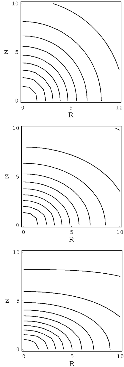
FIG. 1. Halo isodensity contours for the Evans models for q = 1, 0.85, 0.707 , where the z and R axes are in kpc.
