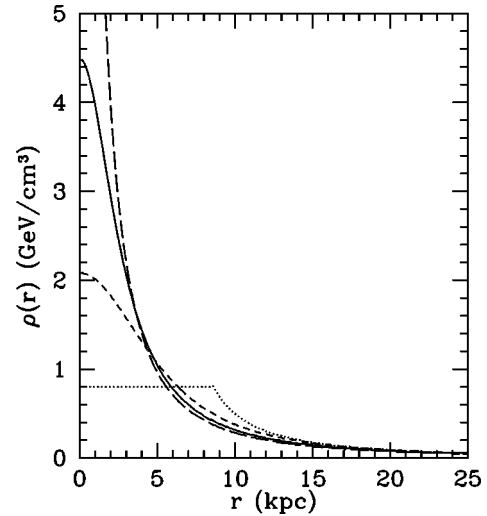
FIG. 7. The radial profile of the three spherical halo models discussed in the text. The solid, short-dash, and long-dash curves are for the canonical isothermal [Eq. (5.1)], spherical Evans [Eq. (5.2)], and alternative isothermal [Eq. (5.3)] models, respectively. The dotted curve is for the nonincreasing radial profile that gives the largest local density.
