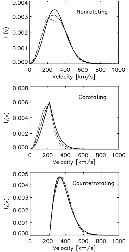
FIG. 2. Local speed distributions f_1(v) for nonrotating, maximally corotating, and maximally counterrotating models with q=1 (solid curves), q=0.85 (dashed curves), and q=0.707 (dotted curves) and with v_s=220 km/s.
