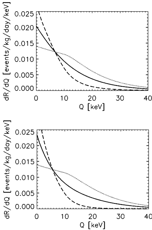
FIG. 3. Differential detection rates for Evans's models q=1 (top) and q=0.707 (bottom) with no net rotation (solid), maximal corotation (dashed), and maximal counterrotation (dotted).
