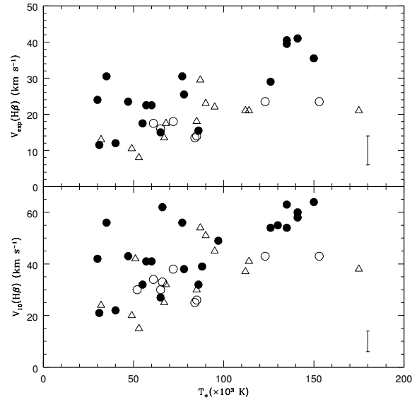
Fig. 6. V_{\text{exp}} (top) and V_{10} (bottom) are plotted versus the stellar temperatures. Symbols are as described in Fig. 4. Despite the large scatter, velocities and temperatures are correlated. The correlations coefficients are 0.64 for the top figure and 0.55 for the bottom figure.
