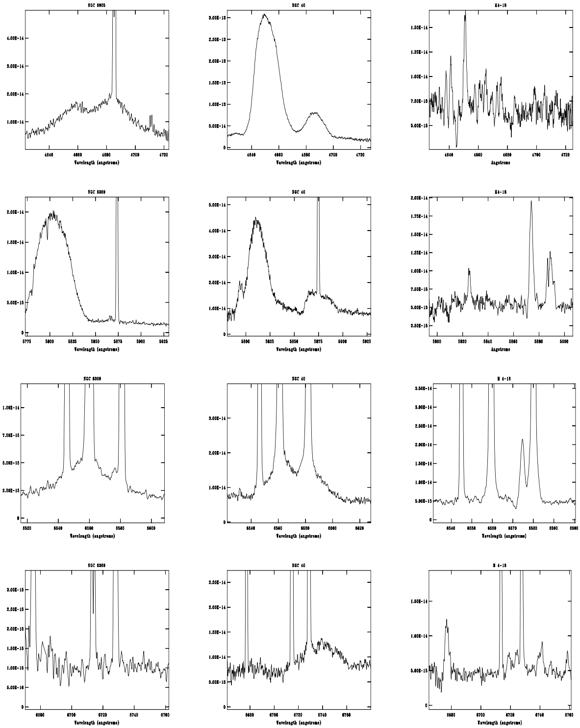
Fig. 9. Profiles of He II \lambda 4686 , He I \lambda 5876 , H\alpha , and [N II] \lambda\lambda 6548, 6583 lines, and [S II] \lambda\lambda 6717, 6731 , showing the nebular and stellar lines for different [WC]-type objects ([WC 2-3] NGC 6905, [WC 4] NGC 6369, [WC 8] NGC 40, [WC 10] M 4-18. The nebular lines can be safely debled from the wide stellar lines even in the cases of slow stellar winds as NGC 40 and M 4-18, except for [N II] \lambda 6583 . [N II] \lambda 6548 can be measured instead. The latter object shows no He II neither He I nebular lines.
