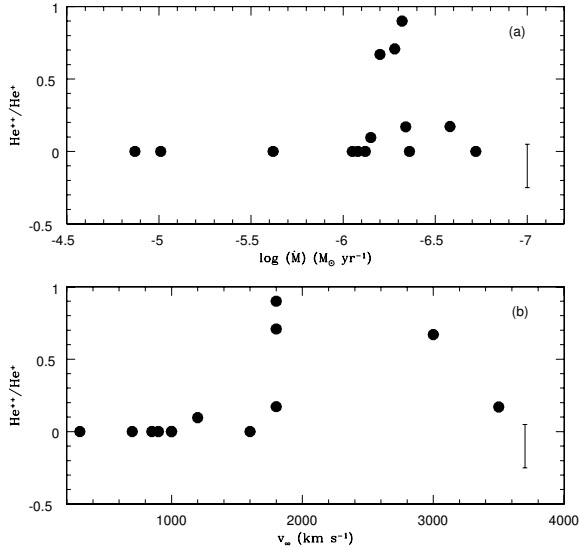
Fig. 7. Nebular ionization degree ( \text{He}^{++}/\text{He}^+ ) is plotted against some stellar parameters such as: a) the mass-loss rate ( \dot{M} ), and b) the wind terminal velocity ( v_\infty ). Symbols are as described in Fig. 4.
