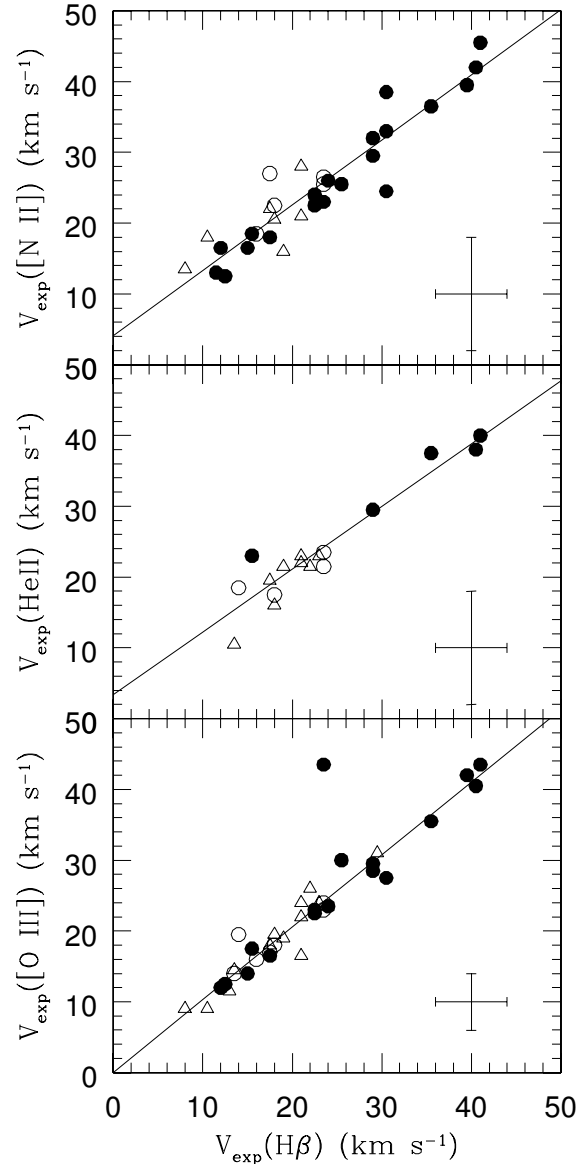
Fig. 4. V_{\text{exp}} from \text{H}\beta are compared to V_{\text{exp}} from: [N II], He II, and [O III]. WRPNe are marked with black circles, WLPNe are marked with open circles and ordinary PNe are marked with open triangles. Least squares fits are shown as solid lines. Typical error bars are shown in each case. The WRPNe conspicuously away from the V_{\text{exp}}([\text{O III}]) versus V_{\text{exp}}(\text{H}\beta) relation is BD+30°3639 which is discussed in Appendix B.
