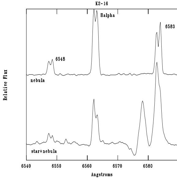
Fig. 10. Nebular only (up) and nebular + stellar (low) extracted spectra in the zone of H\alpha for K 2-16. The nebular spectrum was extracted at about 4-5'' from the central star. The nebular lines show double-peak. The stellar + nebular spectrum shows the intense stellar lines C II lines well mixed with the nebular emission, preventing to measure [N II] \lambda 6583.
