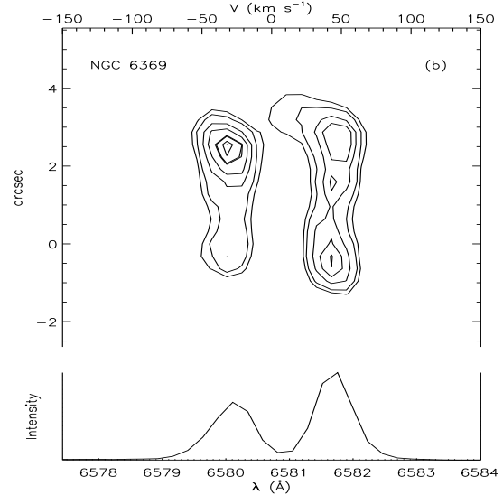
Fig. 11. Position-velocity contours and the extracted spectra from (a) [O III] \lambda 5007 and (b) [N II] \lambda 6583 are shown. The position of the central star is at 0'' in both cases. In (a), the solid line corresponds to the emission of the bright knot at 3'' East from the central star, whereas the dashed double-peak line corresponds to the emission at the central star position (0''). This emission is shown at 5 \times its actual intensity to feature both lines in a single plot. In (b), both emissions at 0'' and 3'' show the same split-line spectrum. The bright knot is not detected in [N II] \lambda 6583.
