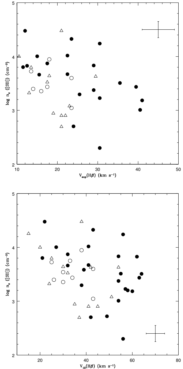
Fig. 5. Electron densities derived from [S II] line ratio are plotted versus V_{\text{exp}} (top) and V_{10} (bottom) from H \beta . Symbols are as described in Fig. 4. Despite the large scatter, both quantities are anticorrelated. The upper open triangle at \log n_e = 4.48 in both panels, corresponds to the young PN NGC 7027.
