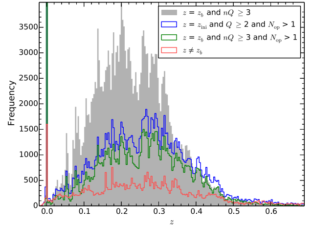
Figure 7. The grey shaded histogram shows the distribution of the finally assigned (i.e. ‘best’) redshifts with nQ \geq 3 for all GAMA II spectra of main survey targets. The green line shows the same but only for those spectra that have been re-redshifted (i.e. those with N_{\text{op}} > 1 ). For these same spectra, the blue line shows the distribution of the initial redshifts with Q \geq 2 . Finally, the red histogram shows the distribution of the redshifts that are not the ‘best’. For clarity, the green and blue histograms have been multiplied by a factor of 3, while the red histogram has been multiplied by 2.
