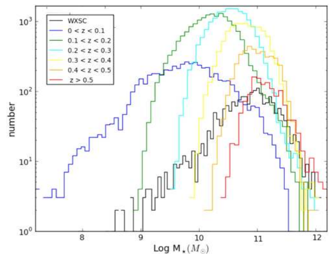
Figure 12. Stellar mass distribution in redshift shells. The lowest mass galaxies detected in GAMA, M_* < 10^9 M_{\odot} , are only seen at low redshifts ( z < 0.1 ) because of the faint surface brightness, while the highest mass galaxies, > 10^{11} M_{\odot} , are seen well beyond the local Universe. For the redshift where GAMA is relatively complete, z < 0.3 , the mass distribution peaks around > 10^{10.5} M_{\odot} .
