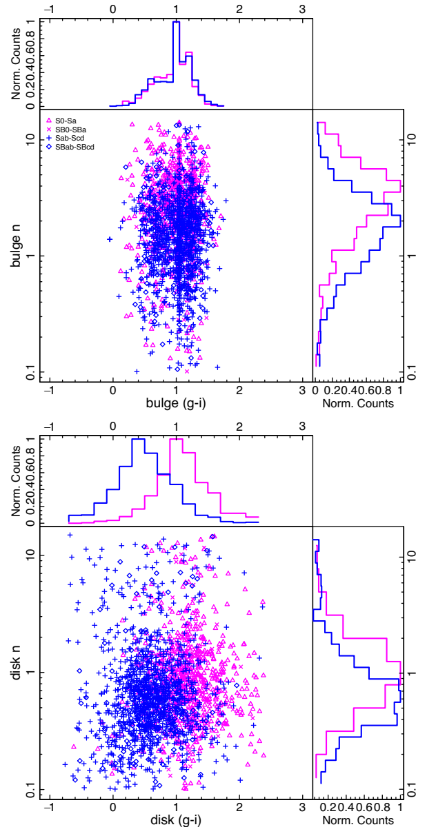
Figure 7. Shown are the (g - i) colour versus Sérsic index distributions for the bulges (top) and discs (bottom) in our two-component galaxy sample. The colour coding in both plots is the same with late types in blue and early types in magenta. The bulges of late-type galaxies have smaller Sérsic indices than the early-type bulges. The Sérsic index distribution of the late-type discs also peaks slightly lower than the early-type discs. Late-type discs are also bluer than early-type discs.
