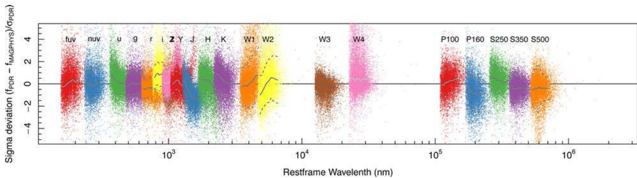
Figure 22. Sigma deviations of the model photometry compared to the input photometry versus rest wavelength for all data points for all galaxies. For each colour, the median and 1\sigma dispersions is measured and shown (grey solid and dotted lines, respectively). The plot shows that the majority of our data lies within the quoted error of the MAGPHYS fits with some outliers (as also noted in Fig. 21). The offset of W4 is of some concern as is the bleeding of the far-IR data towards negative deviation values. Both of these effects are believed to be understood but requires the LAMBDA software (in development). If these are flat and offset it implies a systematic offset, if they show trends with wavelength it implies a progression of a feature with redshift. Trends are most apparent in the near-IR where the modelling of the TP-AGB population is still uncertain.
