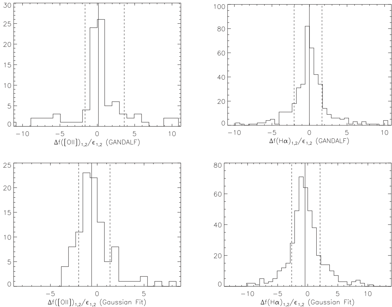
Figure 9. Same as Fig. 7 but the difference is normalized by \epsilon_{1,2} = \sqrt{(\sigma_1^2 + \sigma_2^2)} . If no biases in the measurements exist due to differences in the spectrum S/N , then the distributions should be centred at zero and be symmetric. If the uncertainty estimates are accurate measures of the true uncertainties, then the 68th percentile values should be of the order of unity.
