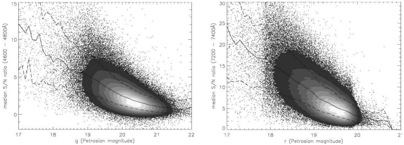
Figure 5. The S/N in the blue (left) and red (right) arms of the GAMA spectra, as a function of g - or r -band Petrosian magnitude, respectively. The solid and dashed lines show the median and 68th percentiles. It is clear that brighter targets have higher S/N, and also that the red arm of the AAOmega spectrograph is relatively more sensitive for a given exposure time. The magnitude limit of r \approx 17.7 mag at the bright end corresponds to the SDSS main galaxy sample limit of r = 17.77 mag. The GAMA selection limit of r = 19.8 mag at the faint end is also apparent. The objects outside these limits include bright targets not observed by SDSS due to fibre-collision limitations, and faint targets included through the additional K - and z -band selection limits (Baldry et al. 2010), together with specific additional filler targets (Ching et al., in preparation).
