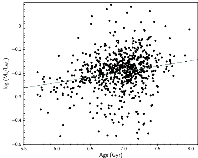
Figure 3. The stellar mass-to-light ratio in the W1 band versus galaxy age t as derived from the T11 optical SED fitting. The straight line shows the overall trend for increasing mass-to-light ratio with age as described in the text.
