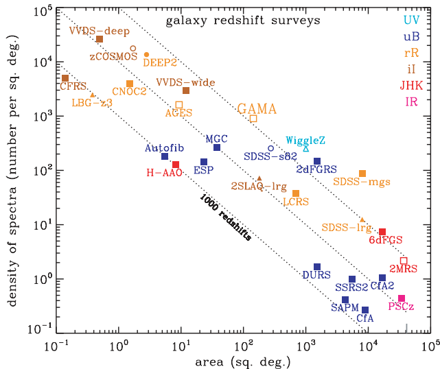
Figure 1. Comparison between field galaxy surveys with spectroscopic redshifts: squares represent predominantly magnitude-limited surveys; circles represent surveys involving colour cuts for photometric redshift selection; while triangles represent highly targeted surveys. The colours represent different principal wavelength selections as in the legend. Filled symbols represent completed surveys. See Table 1 for survey names and references.
