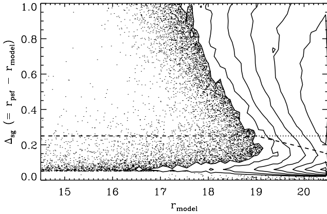
Figure 7. Star–galaxy separation regions. Above \Delta_{sg} = 0.25 , objects are selected as a spectroscopic target regardless of J - K colour (as per AAT observations in 2008 and SDSS MGS). Below the dashed line, objects are selected if they satisfy the J - K star–galaxy separation criteria ( \Delta_{sg,jk} > 0.2 ). While above the dashed line but with \Delta_{sg} < 0.25 (triangular region at r > 19 ), objects are selected if \Delta_{sg,jk} > 0.2 or there is no J - K measurement.
