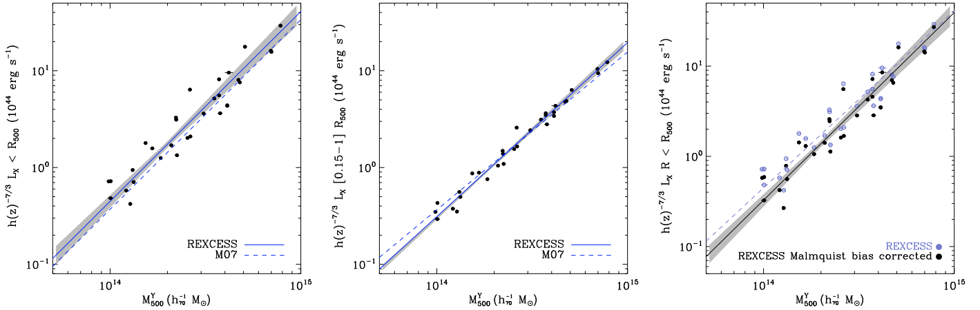
Fig. 6. L – M_{500} relation for the REXCESS sample, with the mass estimated from the Y_X – M relation of Arnaud et al. (2007). Left : relation for all emission interior to R_{500} . Centre : relation for emission in the [0.15\text{--}1] R_{500} aperture. The best fitting power law relation derived from the orthogonal BCES fit method is overlotted as a solid line. The dashed line is the fit derived by Maughan (2007) from observations of 115 galaxy clusters in the Chandra archive. Right : relation corrected for Malmquist bias as described in Appendix B.
