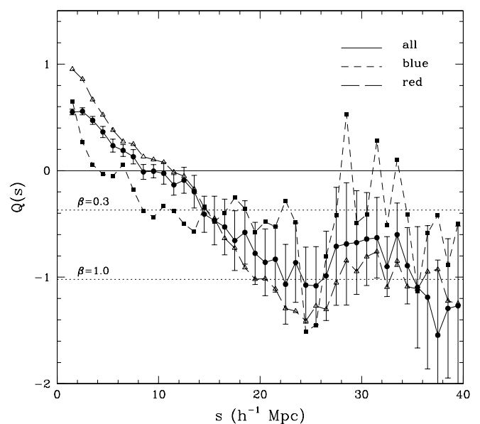
FIG. 14.— Q(s) for the blue (short-dashed line), red (long-dashed line), and full (solid line) samples. For clarity, error bars are drawn only for the full sample.
