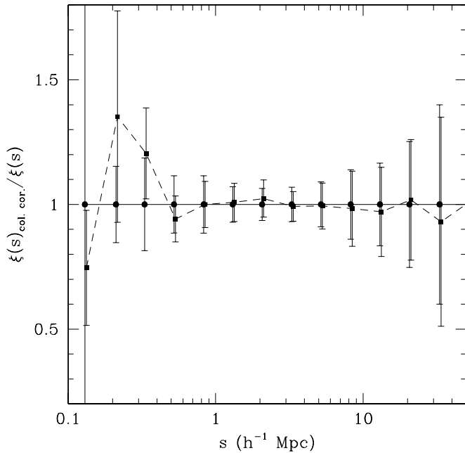
FIG. 3.—Test of the accuracy of our correction for fiber collisions using the tile overlap regions. The dashed line shows the ratio of the redshift-space correlation function measured using the collision-corrected redshifts for all galaxies whose fibers collide to the result obtained using all the available observed redshifts. The latter estimate (and error bars) is given by the solid line at unity. The points and error bars are shifted slightly for clarity.
