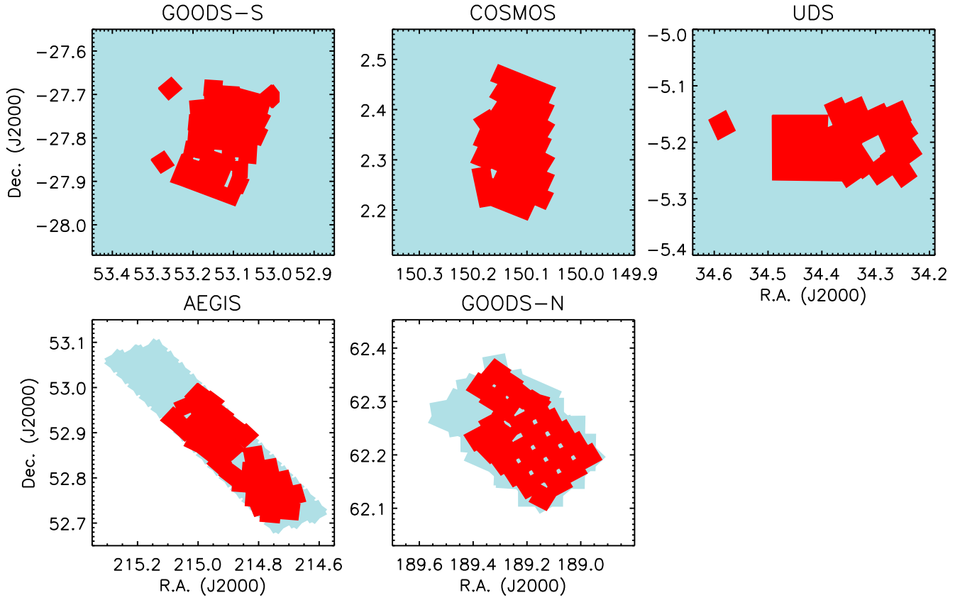
Figure 2. Footprints of the 3D-HST grism observations (red areas) in the five fields studied in this work and of the extended area catalogues (blue areas) used for the edge corrections. White areas have no photometric coverage.
