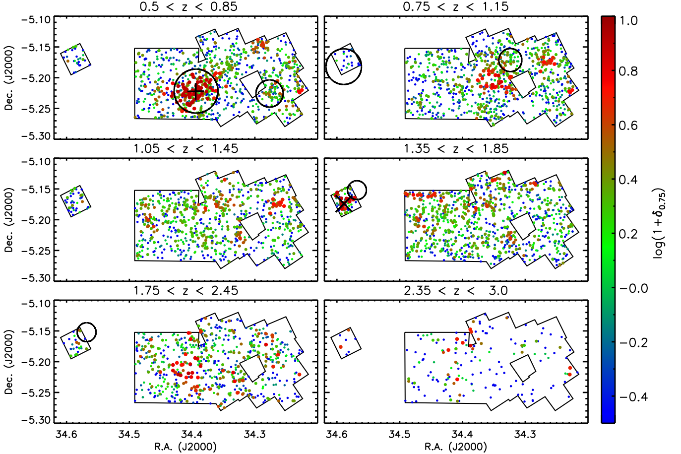
Figure 7. Same as Figure 5 but for the 3D-HST UDS field. The X-Ray extended emission circles (black) are from Finoguenov et al. (2010). The black + and \times symbols mark the center of known clusters at z = 0.65 (Geach et al. 2007, Galametz et al. in prep.) and z = 1.62 (Papovich et al. 2010; Tanaka et al. 2010) respectively.
