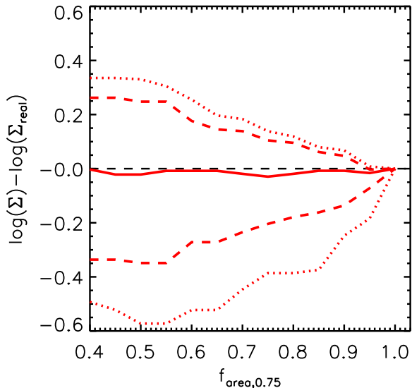
Figure 4. Logarithmic offset between the density ( \Sigma_{\text{real}} ) in a 0.75 Mpc aperture measured using the extended catalogues for COSMOS, GOODS-S, UDS and the density ( \Sigma ) measured using the fraction of the aperture in the 3D-HST footprint ( f_{\text{area},0.75} ) as a function of the latter quantity. The solid line is the median while dashed and dotted lines mark the 1\sigma and 2\sigma confidence intervals respectively. The offset between the two methods is zero, with a scatter which increases with decreasing fraction of the aperture in the 3D-HST footprint.
