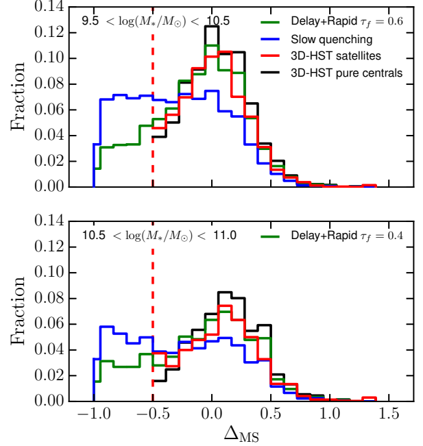
Figure 23. Logarithmic offset from the main sequence ( \Delta_{MS} ) in two stellar mass bins for 3D-HST observed satellites at 0.5 < z < 1.5 (red histogram) and for mock galaxies, in the same redshift range, assuming a “slow quenching” (blue histogram), or a “delayed then rapid” (green histogram) scenario (see text for the details of those two toy models). The histograms are normalized to the total number of 3D-HST satellites (including UVJ passive galaxies). The main sequence offset of a pure sample of observed central galaxies (black histogram) is shown for comparison. The red vertical dashed line is the limit below the main sequence at which SFR estimates for observed galaxies are based predominantly on accurate IR+UV measurements accounting for obscured and unobscured star formation.
