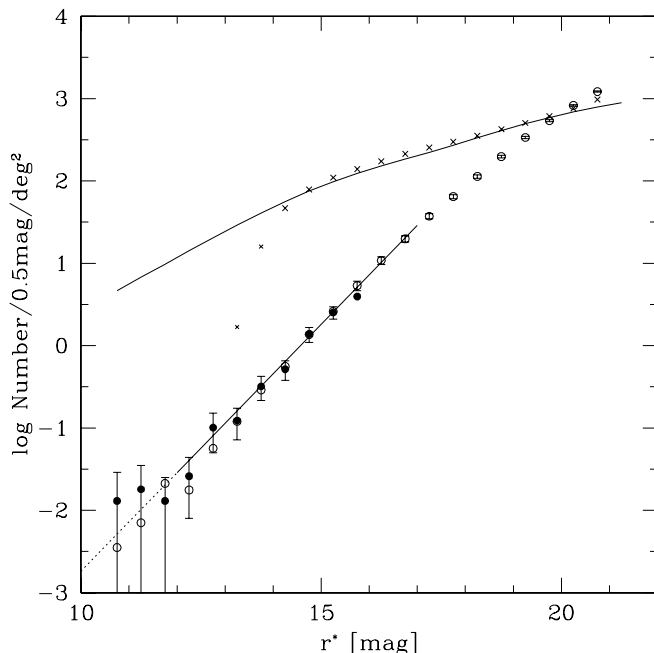
FIG. 4.—Number counts of galaxies as a function of magnitude in the r' band. Filled points show the galaxy counts from the visually inspected sample and open points from the machine-selected sample. The error bars include contributions from both shot-noise and large-scale structure (see text for details). The line segment shows the counts-magnitude relation expected for a homogeneous galaxy distribution in a universe with “Euclidean” geometry: N(r^*) = A_{r^*} 10^{0.6r^*} . The crosses show the observed star counts (small crosses at r^* < 14.5 : data where stars saturate in the SDSS images and therefore suffer from incompleteness). The solid curve shows the prediction of the Bahcall-Soneira model.
