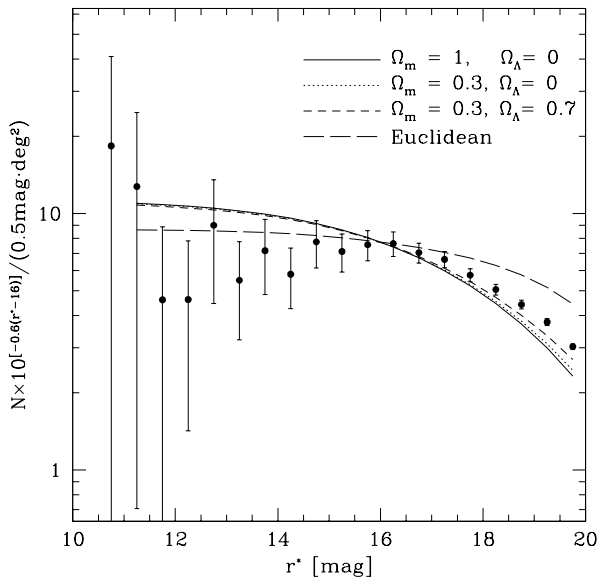
FIG. 6.—Galaxy counts–magnitude relation in the r^* band, normalized by the expected growth rate in a “Euclidean” universe, i.e., N(r^*) \times 10^{-(0.6(r^*-16))} / (0.5 \text{ mag deg}^{-2}) . Points show the observed galaxy counts, while the curves show the predictions of a no-evolution model in three different cosmologies. All the model curves are normalized to the amplitude \tilde{A}_{r^*} derived using equation (10).
