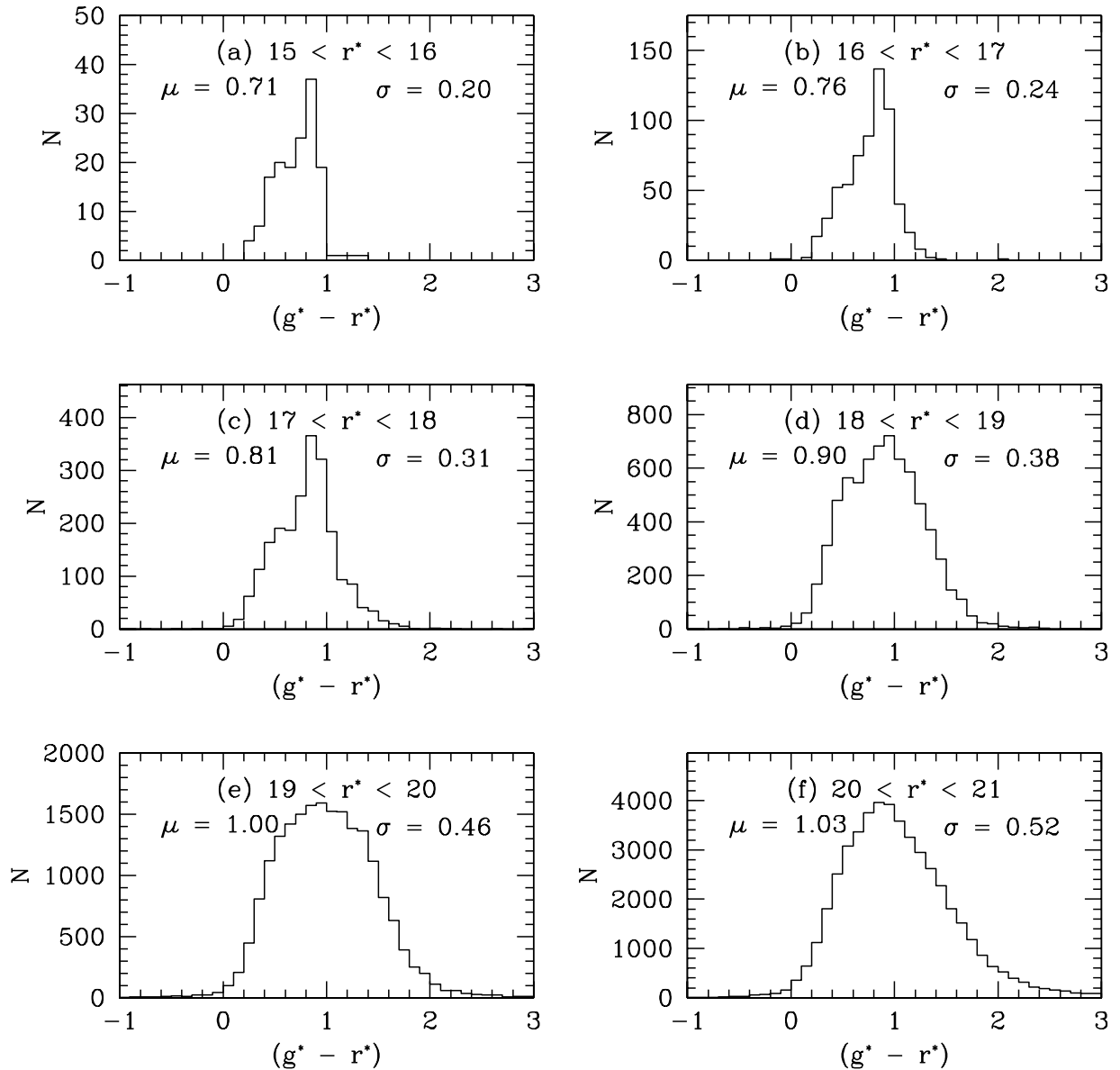
FIG. 14.—Distribution of g^* - r^* colors of all galaxies in the third CCD column of run 756. The colors are computed from the dereddened Petrosian magnitudes of galaxies. (a) to (f): This distribution in different bins of r^* Petrosian magnitude. The mean ( \mu ) and scatter ( \sigma ) of the distribution are listed in each panel.
