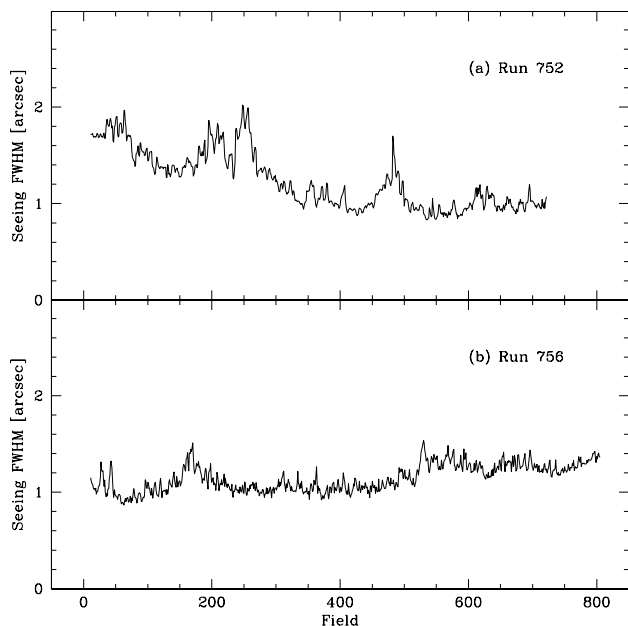
FIG. 1.—Field-to-field variation of seeing (FWHM) in the r' band in the third CCD column during TDI observations: (a) run 752, extending for 7 hr; (b) run 756, extending for 8 hr.
