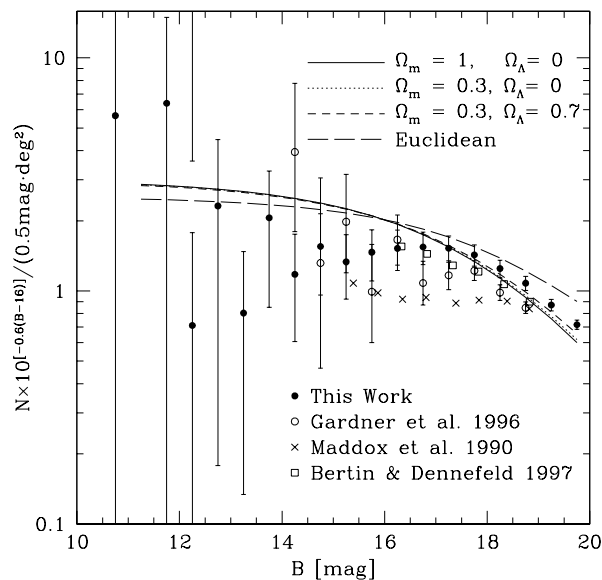
FIG. 10.—Galaxy counts–magnitude relation in the B band normalized by the expected growth rate in a “Euclidean” universe, i.e., N(B) \times 10^{(-0.6(B-16))} . Filled points show the observed galaxy counts from this work, while the curves show the predictions of a no-evolution model in three different cosmologies. All the model curves are normalized to the amplitude \bar{A}_B of the data. The open circles, crosses, and open squares show the data on galaxy counts in B band from three previous studies.
