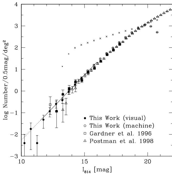
FIG. 11.—Number counts of galaxies as a function of magnitude in the I_{814} band, using the color transformation given in eq. (12). Filled circles show the galaxy counts from the visually inspected sample, and open circles from the machine-selected sample. The error bars include contributions from both shot-noise and large-scale structure. The line segment shows the counts-magnitude relation expected in a homogeneous universe with “Euclidean” geometry: N(I) = A_I 10^{0.6I} . The crosses show the observed star counts. The squares and triangles show galaxy counts from previous studies.
