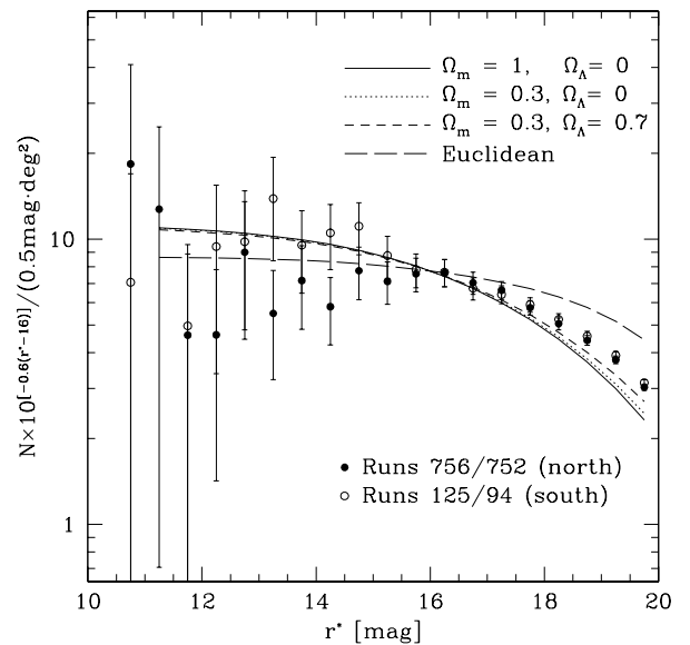
FIG. 12.—Galaxy counts–magnitude relation in the r^* band normalized by the expected growth rate in a “Euclidean” universe, i.e., N(r^*) \times 10^{[-0.6(r^*-16)]} . Filled points show the galaxy counts from the northern equatorial stripe, and open points show the counts from the southern equatorial stripe. The curves show the predictions of a no-evolution model in three different cosmologies. The model curves are normalized to the amplitude \tilde{A}_{r^*} of the data from the northern equatorial stripe.
