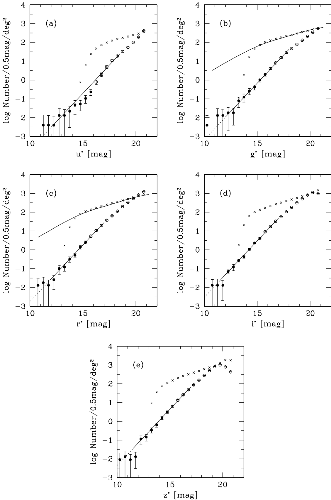
FIG. 7.—Number counts of galaxies as a function of magnitude in the five color bands u^* , g^* , r^* , i^* , and z^* for the northern equatorial stripe. Filled points show the galaxy counts from the visually inspected sample, and open points from the machine-selected sample. The error bars include contributions from both shot-noise and large-scale structure (see text for details). The line segment shows the counts-magnitude relation expected in a homogeneous universe with “Euclidean” geometry: N(m) = A_i 10^{0.6m} . The crosses show the observed star counts ( small crosses : data where stars saturate in the image and therefore suffer from incompleteness), and the solid curve shows the prediction of the Bahcall-Soneira model.
