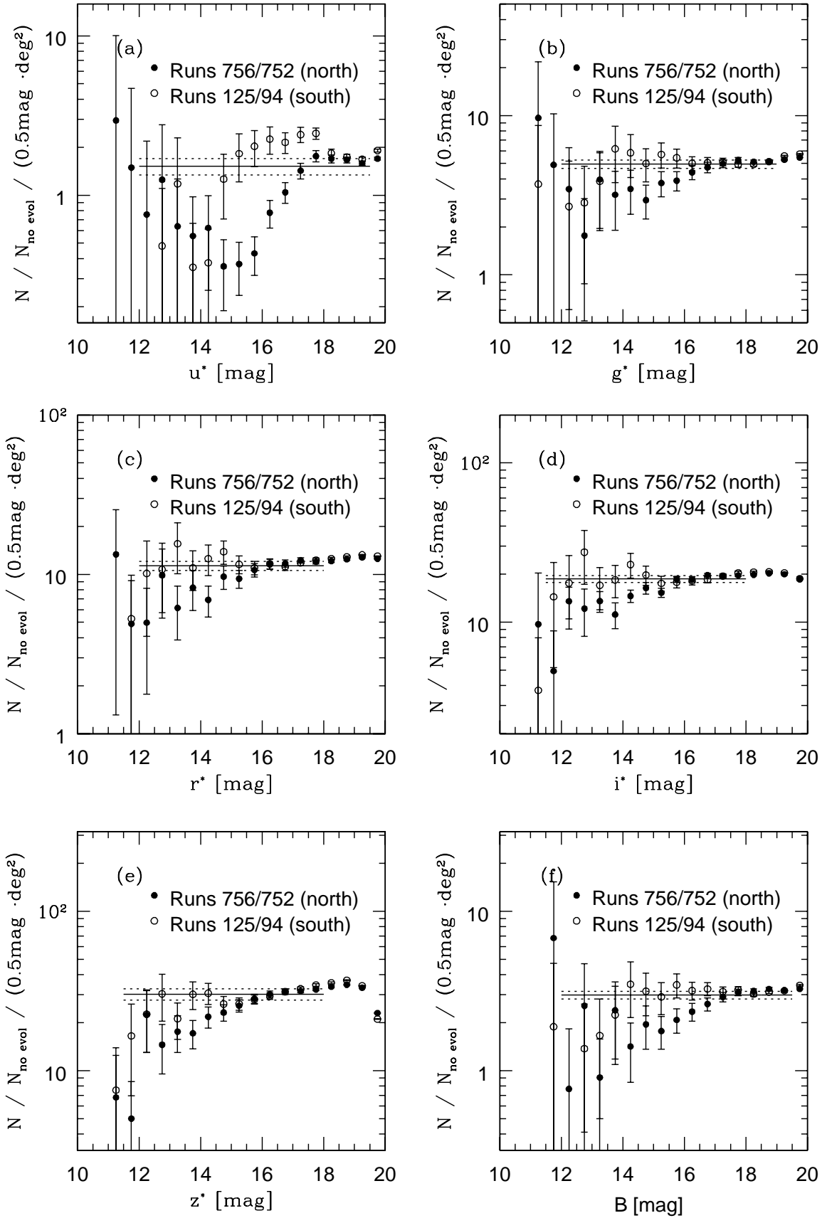
FIG. 8.—Galaxy counts–magnitude relation in the u^* , g^* , r^* , i^* , z^* , and B bands, normalized by the no-evolution model prediction N(\lambda)_{\text{no evol}} . Filled points show the observed galaxy counts from the northern equatorial stripe, and open points are those from the southern equatorial stripe as discussed in § 8. The solid lines correspond to \bar{A}_{\lambda^*} , and dotted lines show 1\sigma error ranges.
