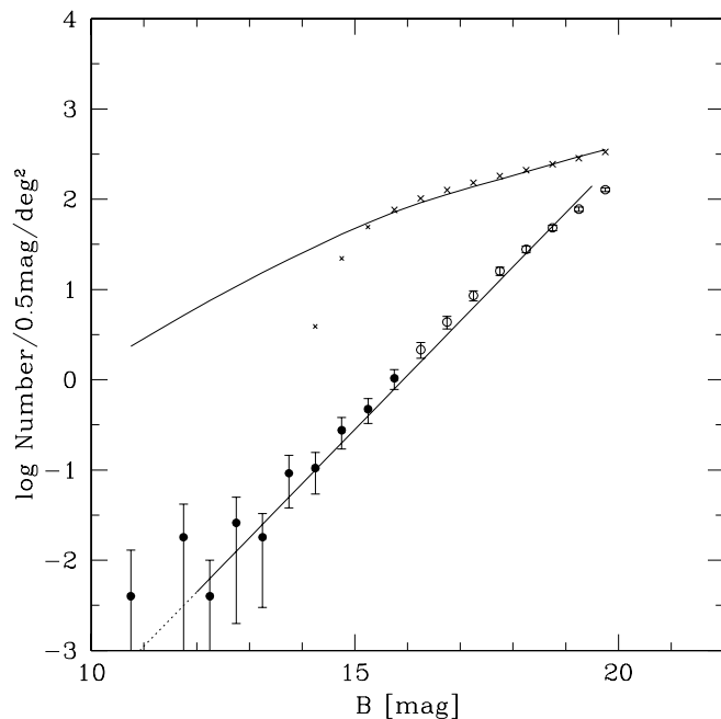
FIG. 9.—Number counts of galaxies as a function of magnitude in the B band, using the color transformation given in eq. (11). Filled points show the galaxy counts from the visually inspected sample, and open points from the machine-selected sample. The error bars include contributions from both shot-noise and large-scale structure (see text for details). The line segment shows the counts-magnitude relation expected in a homogeneous universe with “Euclidean” geometry: N(B) = A_B 10^{0.6B} . The crosses show the observed star counts ( small crosses : data where stars saturate in the image and therefore suffer from incompleteness), and the solid curve shows the prediction of the Bahcall-Soneira model.
