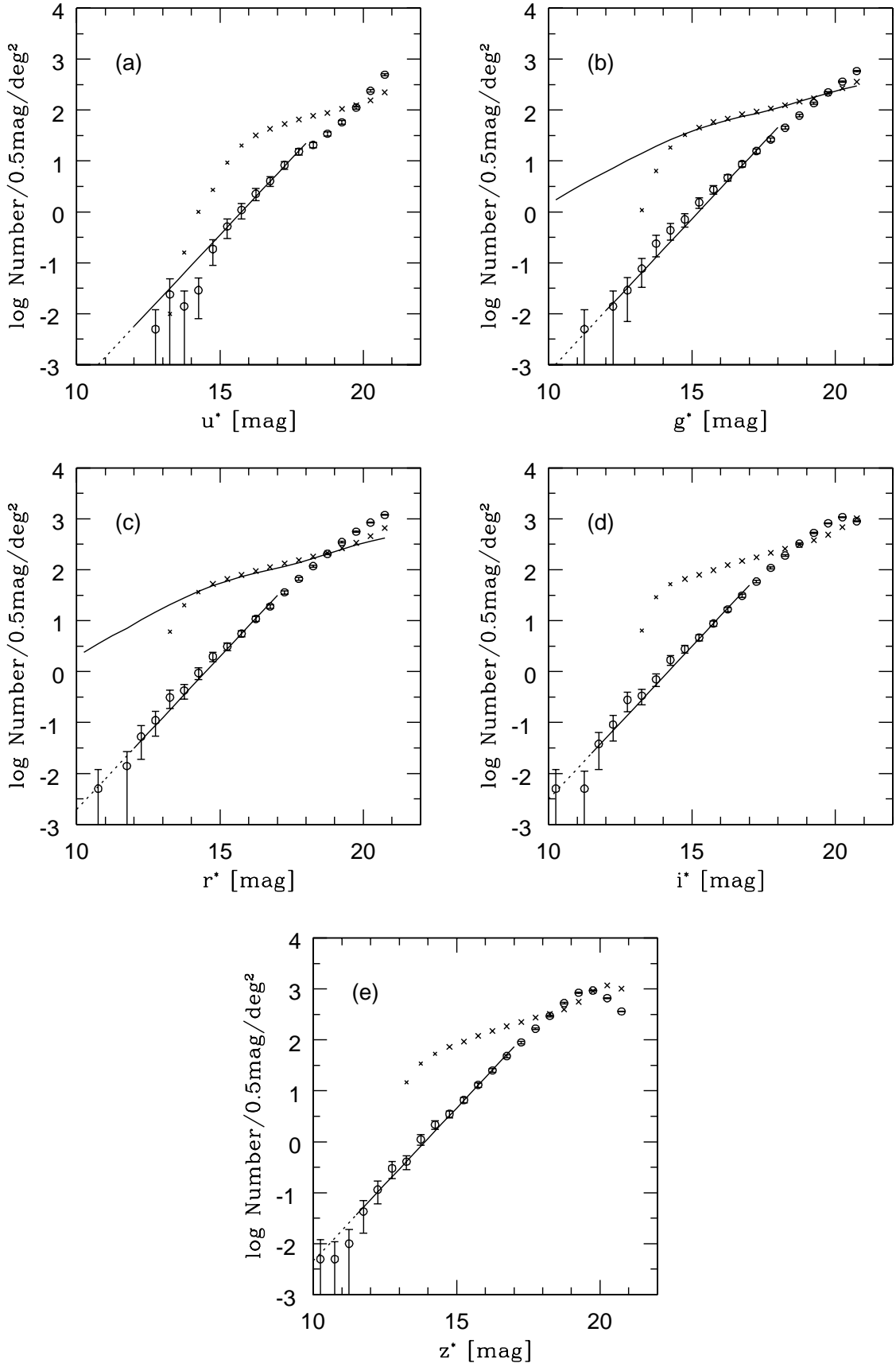
FIG. 13.—Number counts of galaxies as a function of magnitude in the five color bands u^* , g^* , r^* , i^* , and z^* for the southern equatorial stripe. Open points show the galaxy counts from the machine-selected sample. The error bars include contributions from both shot-noise and large-scale structure (see text for details). The line segment shows the counts-magnitude relation expected in a homogeneous universe with “Euclidean” geometry: N(m) = A_s 10^{0.6m} . The crosses show the observed star counts ( small crosses : data where stars saturate in the image and therefore suffer from incompleteness), and the solid curve shows the prediction of the Bahcall-Soneira model.
