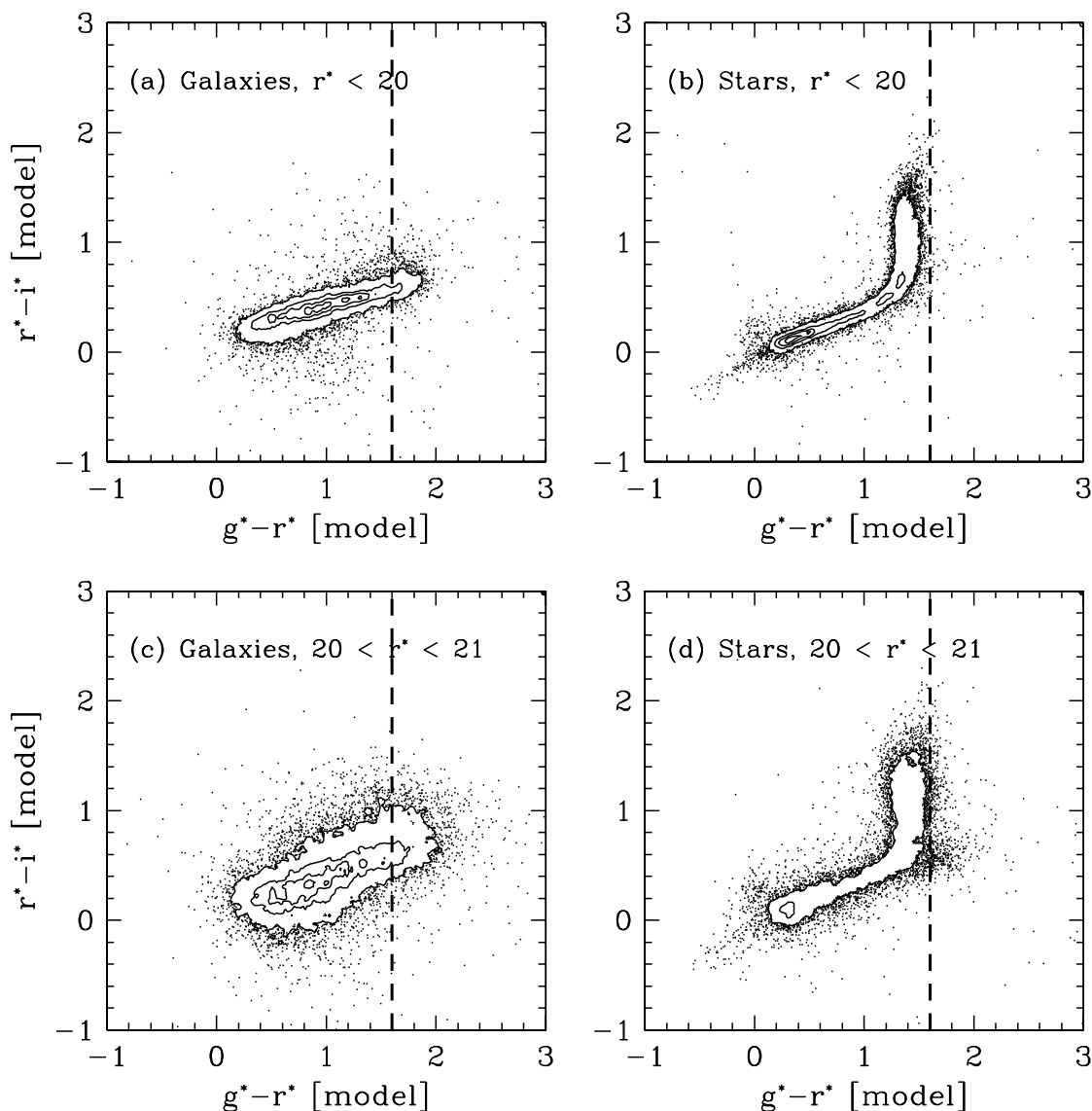
FIG. 2.—Distribution in the g^*-r^* , r^*-i^* plane of all objects classified as galaxies and stars in fields 251 to 300 of the third CCD column of run 756. (The star sample contains 50–100 quasars.) The inner parts of the distributions are shown as contours, linearly spaced in the density of objects in the color-color plane. (a) and (b): Distribution of objects classified as galaxies and stars, respectively, in the magnitude range 16 < r^* < 20 . (c) and (d): Corresponding objects in the magnitude range 20 < r^* < 21 . Objects in (b) and (d) with g^*-r^* > 1.6 (dashed line) are real galaxies that are misclassified as stars, quasars, or stars with incorrect photometry.
