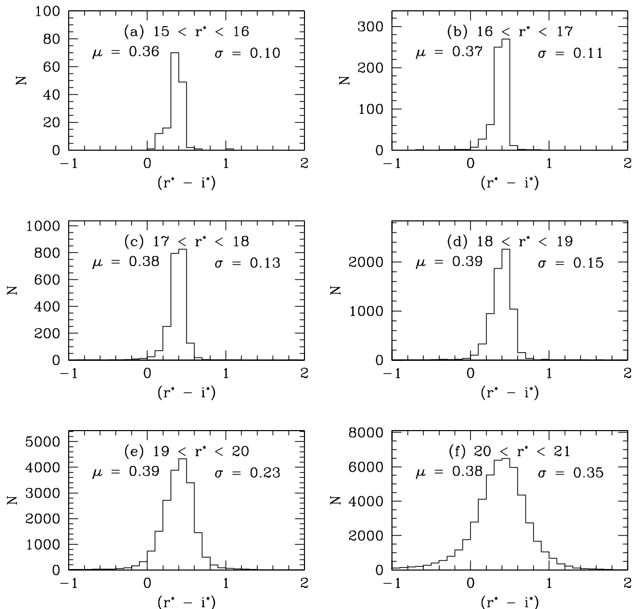
FIG. 15.—Distribution of r^* - i^* colors of all galaxies in the third CCD column of run 756. The colors are computed from the dereddened Petrosian magnitudes of galaxies. (a) to (f): This distribution in different bins of r^* Petrosian magnitude. The mean ( \mu ) and scatter ( \sigma ) of the distribution are listed in each panel.
